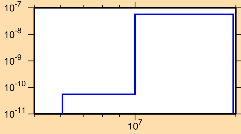
\sigma vs. E for ^{189}\text{Au}(n,p\alpha)
