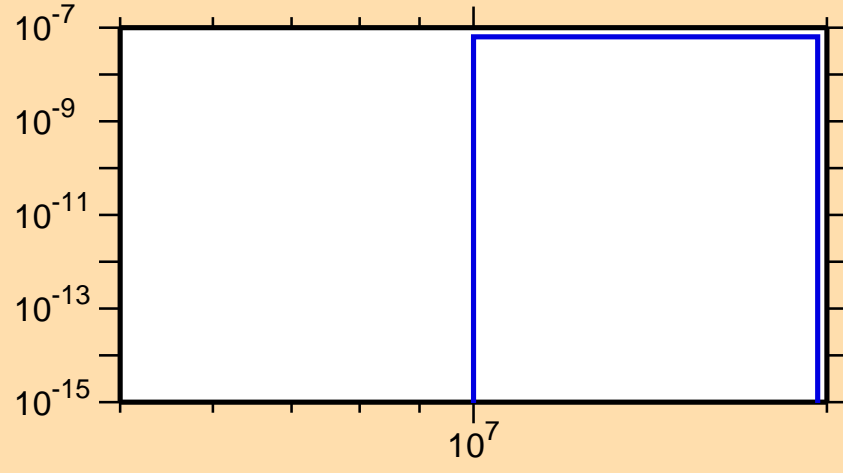
\sigma vs. E for ^{189}\text{Au}(n,2n\alpha)
