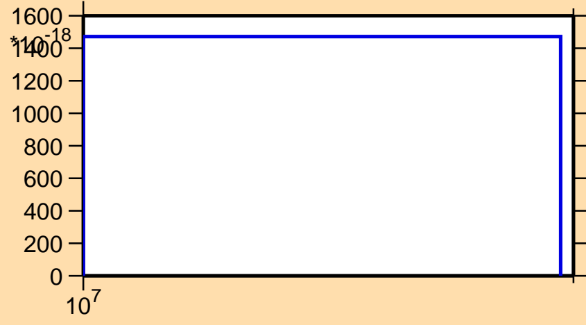
\sigma vs. E for ^{189}\text{Au} (mt 34)
