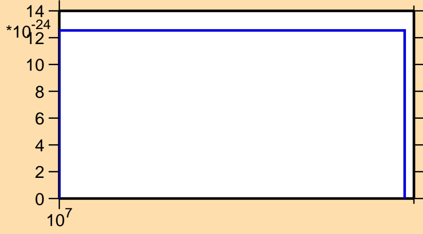
\sigma vs. E for ^{189}\text{Au} (mt 42)
