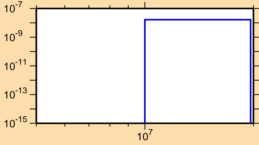
\sigma vs. E for ^{189}\text{Au}(n,\text{He}3)
