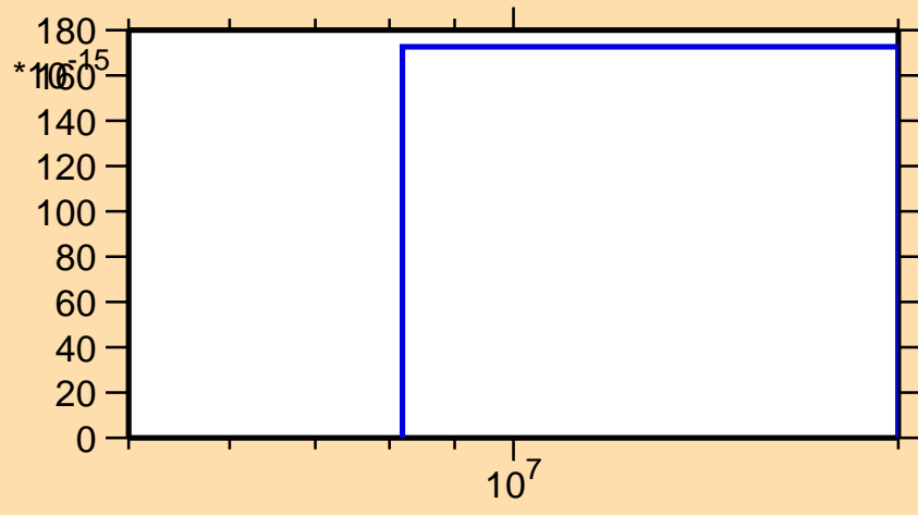
\sigma vs. E for ^{189}\text{Au}(n,pd)
