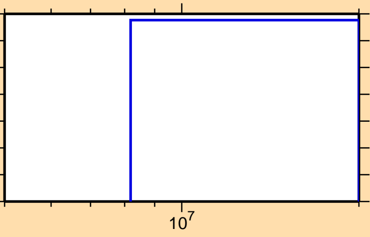
\sigma vs. E for ^{189}\text{Au}(n,\text{He}3)
