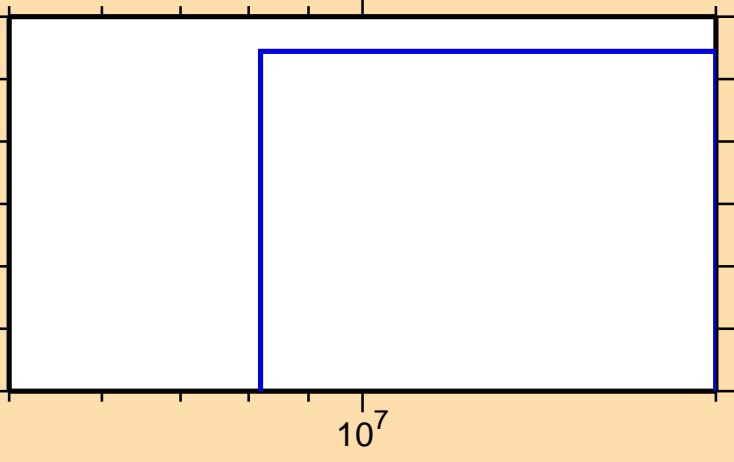
\sigma vs. E for ^{189}\text{Au}(n,nd)
