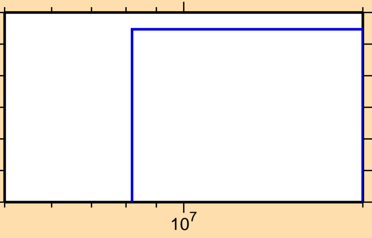
\sigma vs. E for ^{189}\text{Au}(n,nt)
