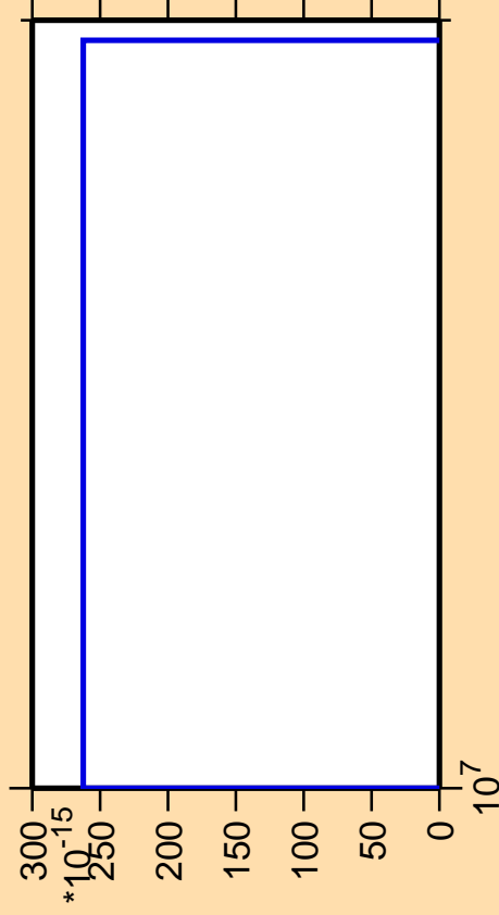
\Delta\sigma/\sigma vs. E for ^{191}\text{Au} (mt 42)
