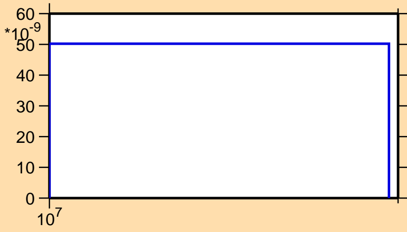
\sigma vs. E for ^{191}\text{Au}(n,2np)
