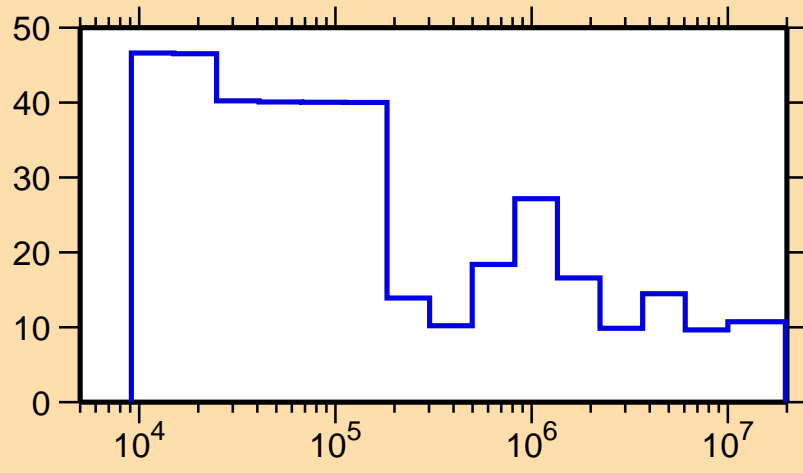
\Delta\sigma/\sigma vs. E for ^{191}\text{Au}(n,\text{tot.})
