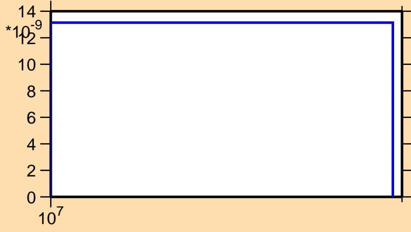
\sigma vs. E for ^{191}\text{Au}(n,\text{nd})
