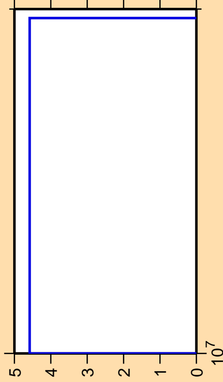
\Delta\sigma/\sigma vs. E for ^{191}\text{Au}(\text{mt117})
