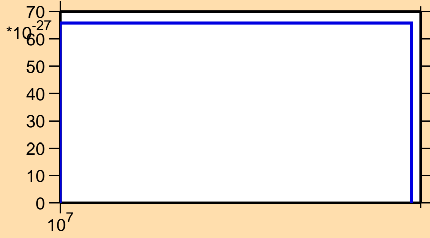
\sigma vs. E for ^{191}\text{Au} (mt 42)
