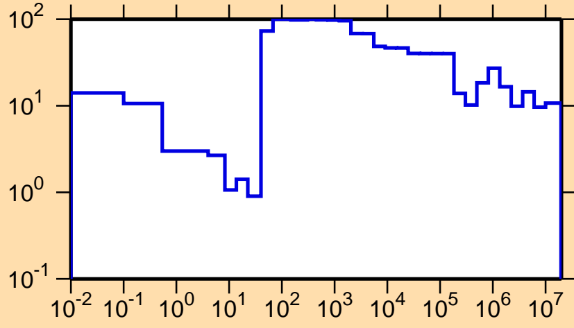
\Delta\sigma/\sigma vs. E for ^{191}\text{Au}(n,\text{tot.})
