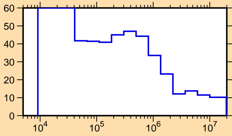
\Delta\sigma/\sigma vs. E for ^{191}\text{Au}(n,\text{nonel.})
