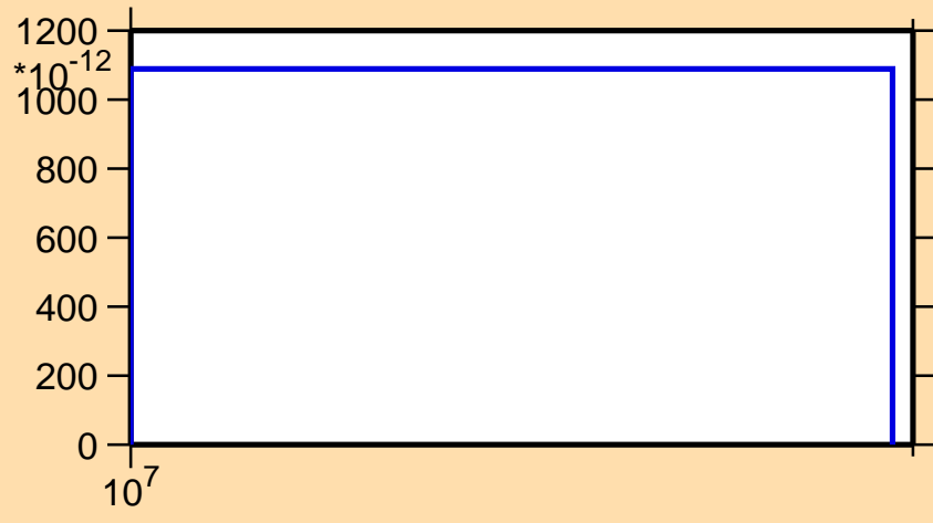
\sigma vs. E for ^{191}\text{Au}(n,\text{He}3)
