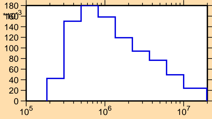
\sigma vs. E for ^{191}\text{Au}(n,n_2)
