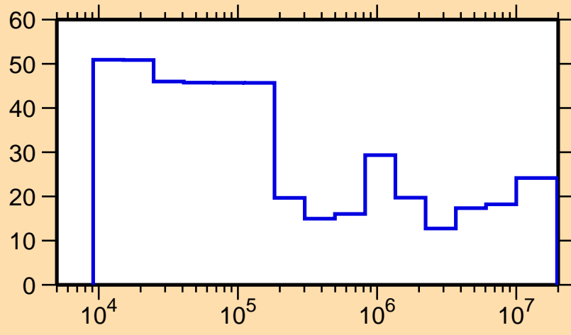
\Delta\sigma/\sigma vs. E for ^{191}\text{Au}(n,\text{el.})
