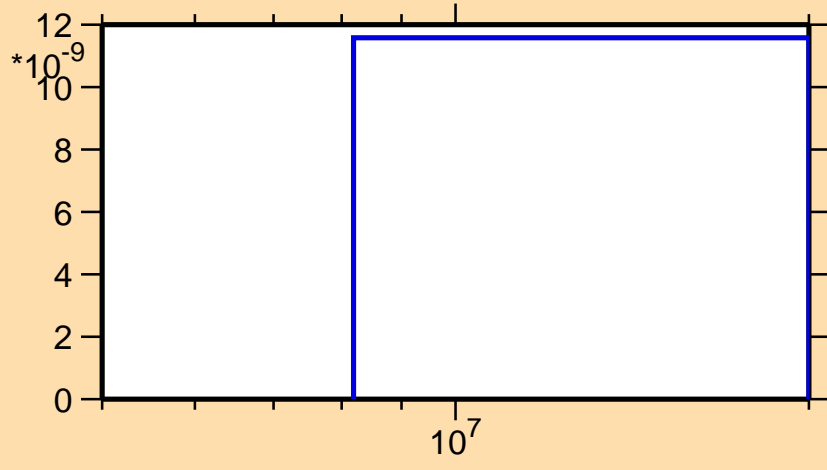
\sigma vs. E for ^{191}\text{Au}(n,nd)
