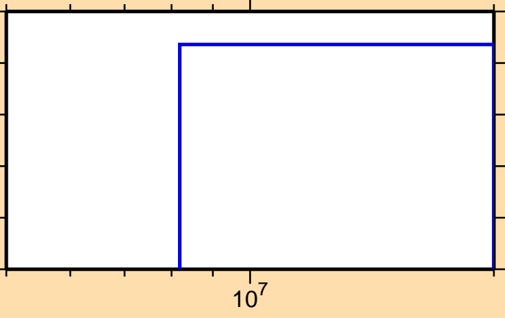
\sigma vs. E for ^{191}\text{Au}(n,nt)
