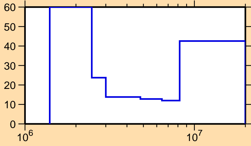
\Delta\sigma/\sigma vs. E for ^{191}\text{Au}(n,n\text{cont.})
