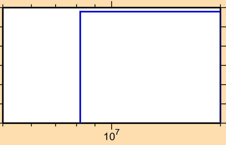
\sigma vs. E for ^{191}\text{Au}(n,nd)
