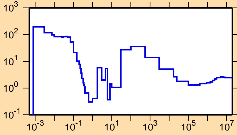
\sigma vs. E for ^{191}\text{Au}(n,\text{nonel.})
