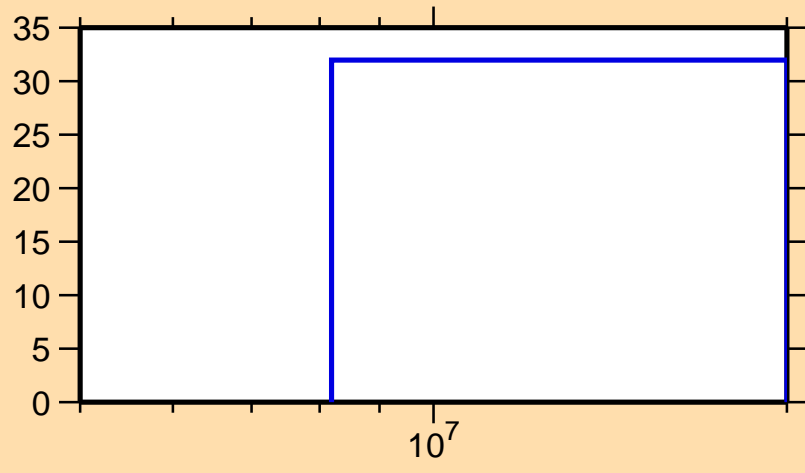
\Delta\sigma/\sigma vs. E for ^{191}\text{Au}(n,2n)
