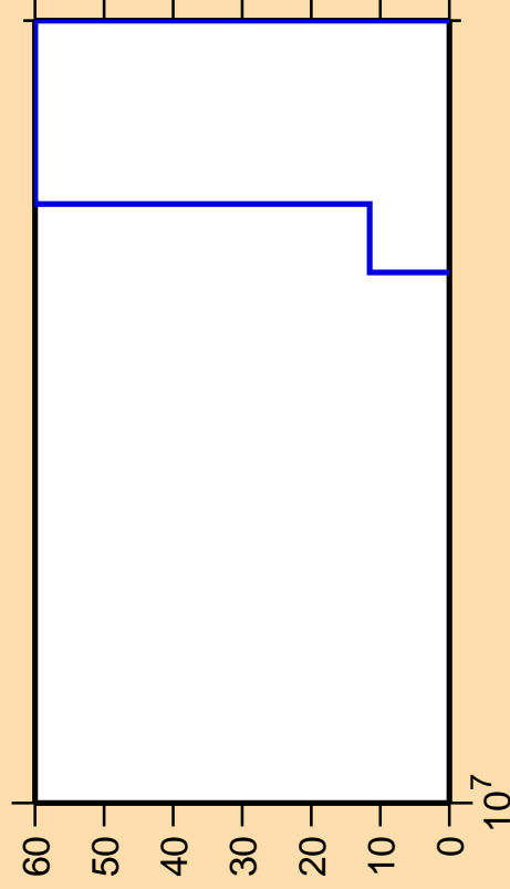
\Delta\sigma/\sigma vs. E for ^{192}\text{Au} (mt 45)
