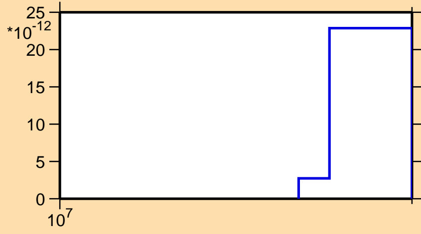
\sigma vs. E for ^{192}\text{Au} (mt 45)
