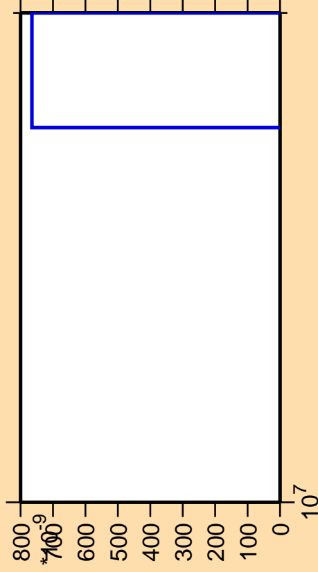
\Delta\sigma/\sigma vs. E for ^{192}\text{Au} (mt 42)
