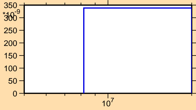
\sigma vs. E for ^{192}\text{Au}(n,nd)
