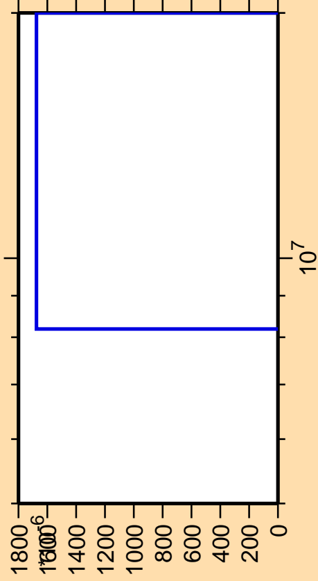
\Delta\sigma/\sigma vs. E for ^{192}\text{Au}(n,\text{pd})
