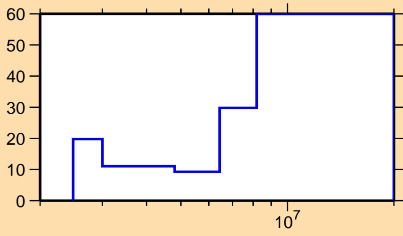
\Delta\sigma/\sigma vs. E for ^{192}\text{Au}(n,n\text{cont.})
