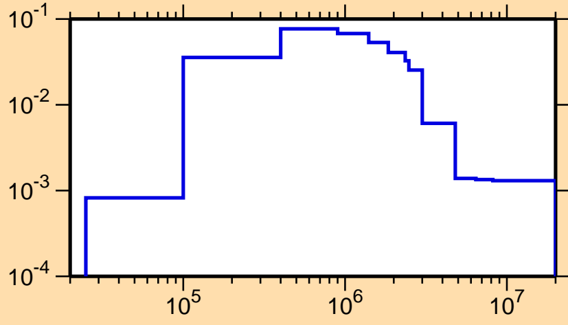
\sigma vs. E for ^{192}\text{Au}(n,n_2)
