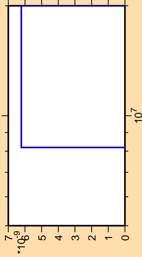
\Delta\sigma/\sigma vs. E for ^{192}\text{Au}(\text{mt } 42)
