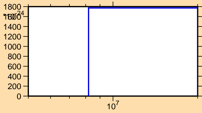
\sigma vs. E for ^{192}\text{Au}(\text{mt } 42)
