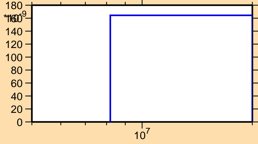
\sigma vs. E for ^{192}\text{Au}(n,2n\alpha)
