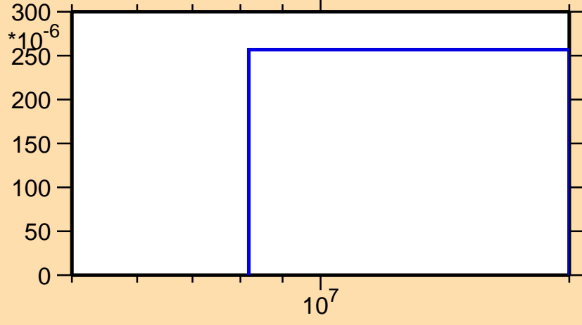
\sigma vs. E for ^{192}\text{Au}(n,3n)
