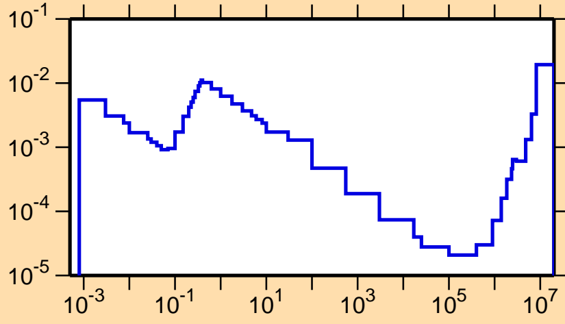
\sigma vs. E for ^{192}\text{Au}(n,p)
