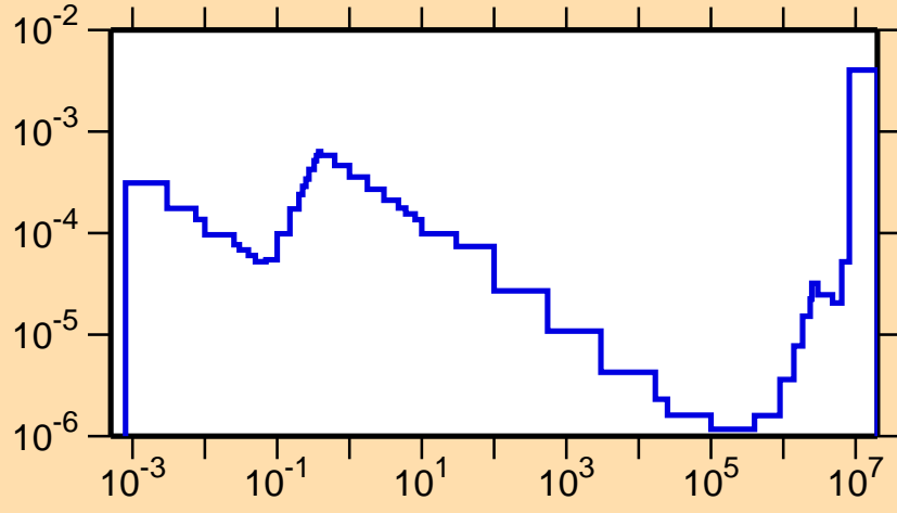
\sigma vs. E for ^{192}\text{Au}(n,\alpha)
