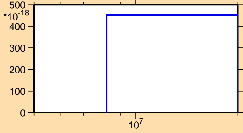
\sigma vs. E for ^{192}\text{Au}(n,\text{pd})
