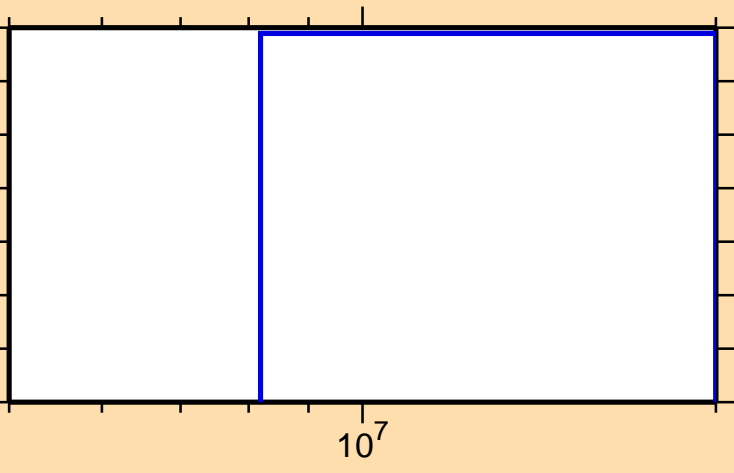
\sigma vs. E for ^{193}\text{Au}(n,3n)
