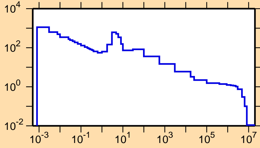
\sigma vs. E for ^{193}\text{Au}(n,\gamma)
