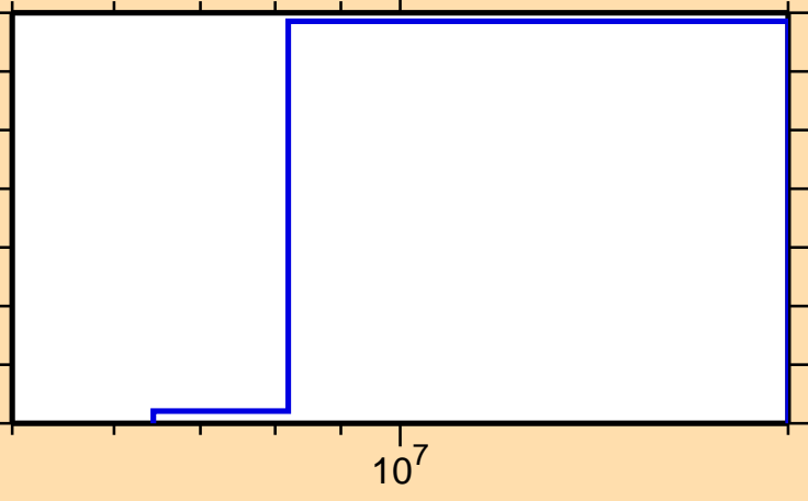
\sigma vs. E for ^{193}\text{Au}(n,d)
