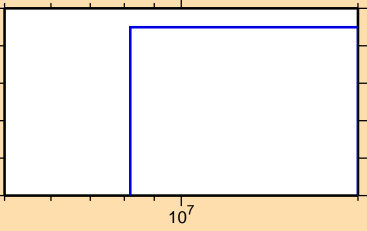
\sigma vs. E for ^{193}\text{Au}(n,2np)
