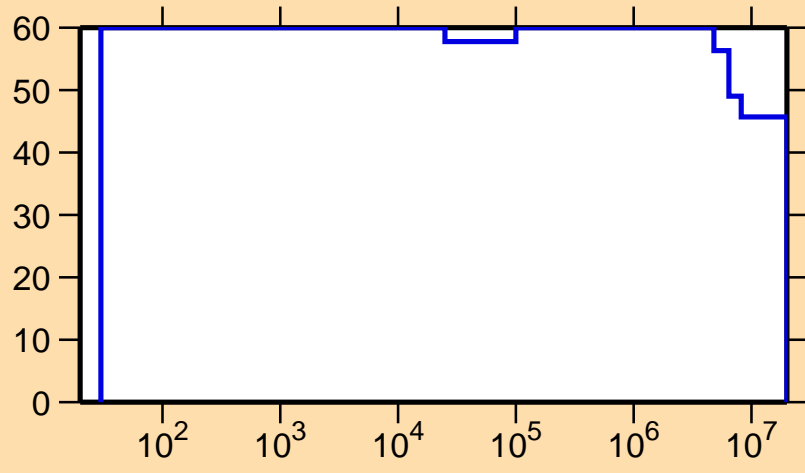
\Delta\sigma/\sigma vs. E for ^{193}\text{Au}(n,n_1)
