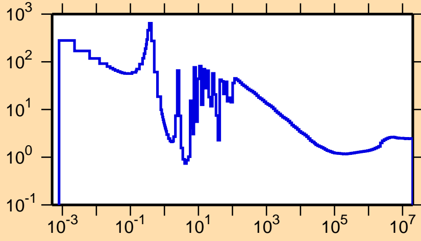
\sigma vs. E for ^{194}\text{Au}(n,\text{nonel.})
