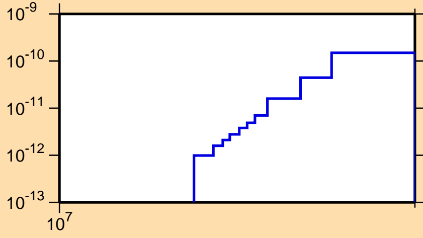
\sigma vs. E for ^{194}\text{Au}(n,p\alpha)
