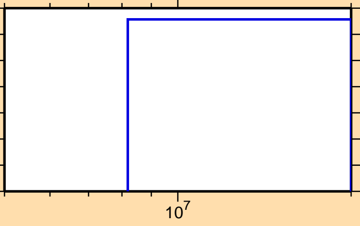
\sigma vs. E for ^{194}\text{Au}(n,2n\alpha)
