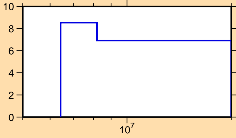
\Delta\sigma/\sigma vs. E for ^{194}\text{Au}(n,\text{nonel.})
