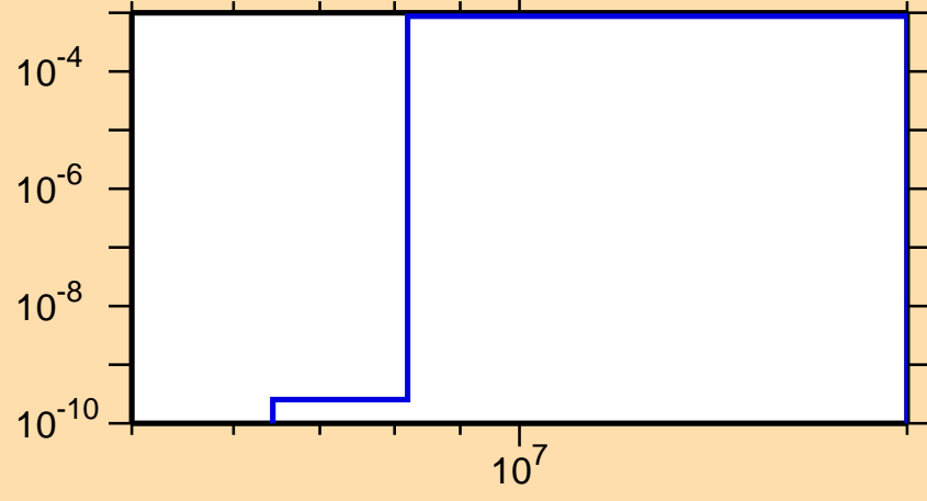
\sigma vs. E for ^{194}\text{Au}(n,np)
