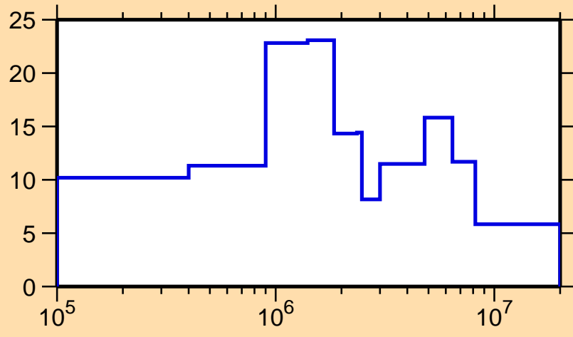
\Delta\sigma/\sigma vs. E for ^{194}\text{Au}(n,\text{el.})
