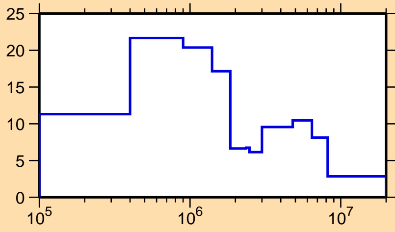
\Delta\sigma/\sigma vs. E for ^{194}\text{Au}(n, \text{tot.})
