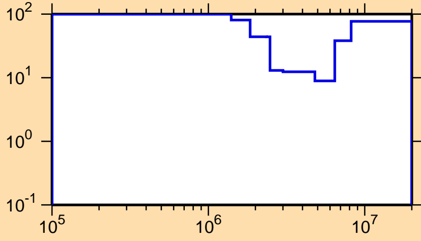
\Delta\sigma/\sigma vs. E for ^{194}\text{Au}(n,n\text{cont.})
