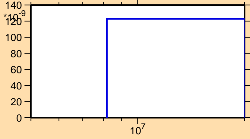
\sigma vs. E for ^{194}\text{Au}(n,nd)
