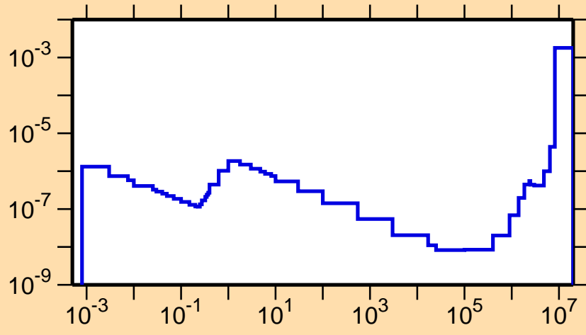
\sigma vs. E for ^{194}\text{Au}(n,\alpha)
