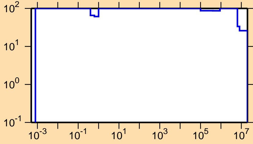
\Delta\sigma/\sigma vs. E for ^{194}\text{Au}(n,p)
