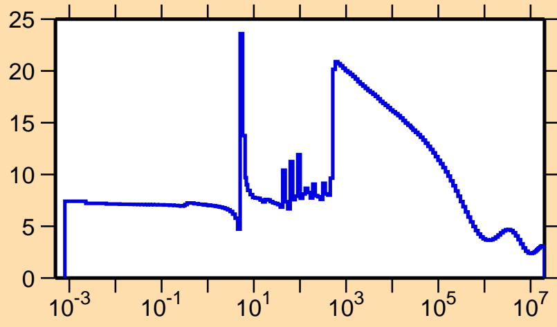
\sigma vs. E for ^{195}\text{Au}(n,\text{el.})
