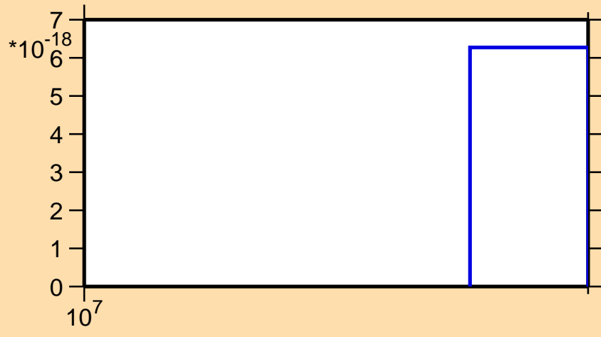
\sigma vs. E for ^{195}\text{Au} (mt 42)
