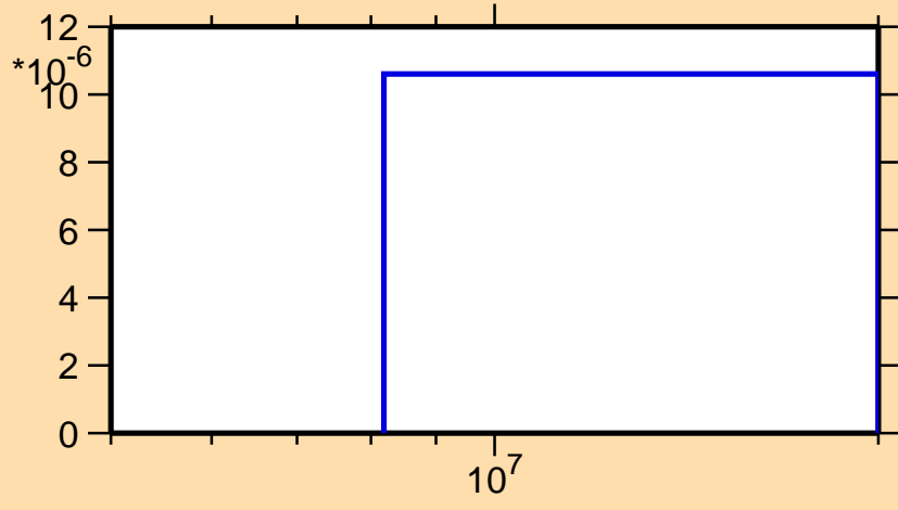
\sigma vs. E for ^{195}\text{Au}(n,t)
