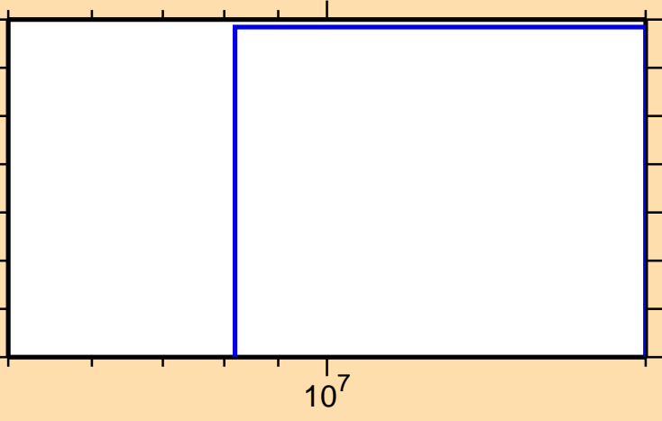
\sigma vs. E for ^{195}\text{Au}(n,p\alpha)
