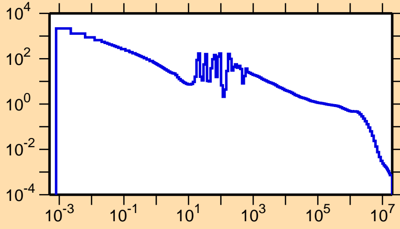
\sigma vs. E for ^{197}\text{Au}(n,\gamma)
