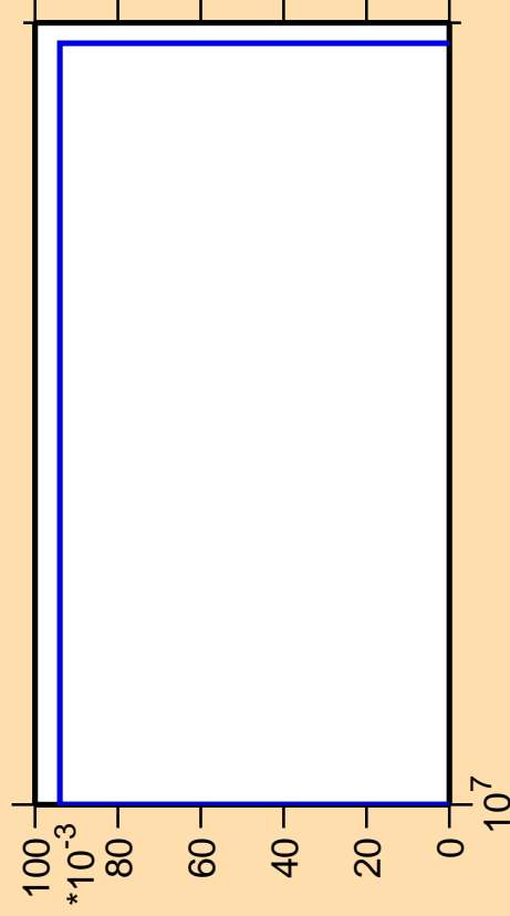
\Delta\sigma/\sigma vs. E for ^{197}\text{Au}(n,\text{He}3)
