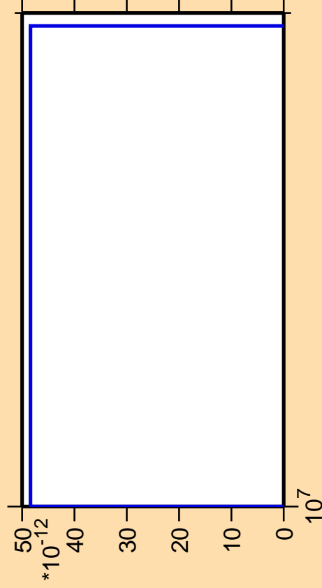
\Delta\sigma/\sigma vs. E for ^{197}\text{Au} (mt 42)
