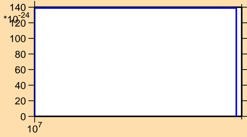
\sigma vs. E for ^{197}\text{Au} (mt 42)
