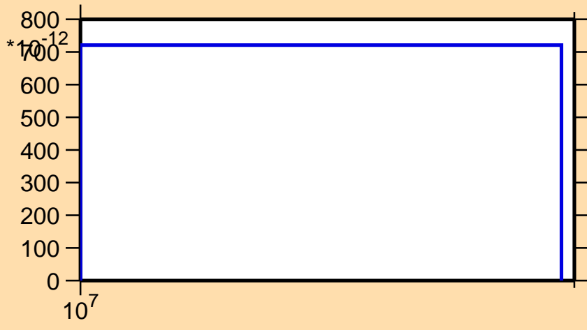
\sigma vs. E for ^{197}\text{Au}(n,nt)
