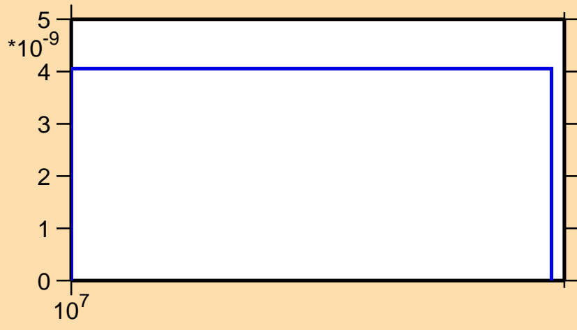
\sigma vs. E for ^{197}\text{Au}(n,\text{nd})
