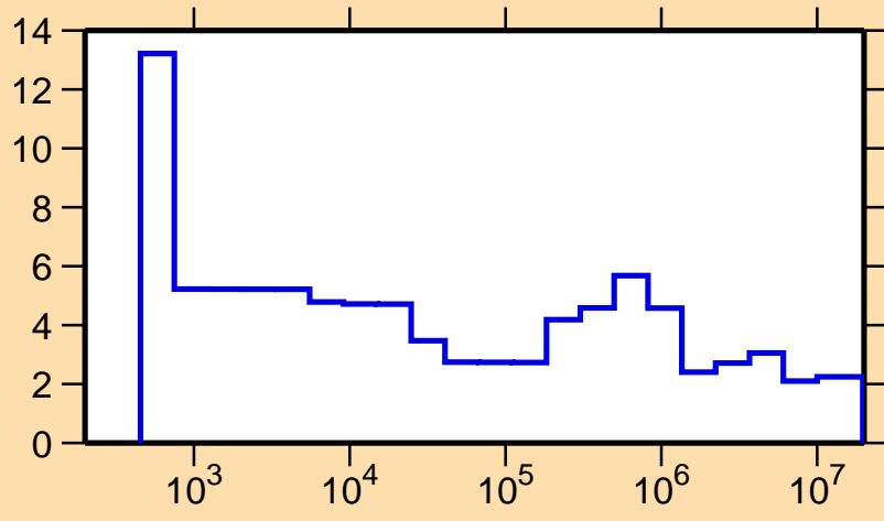
\Delta\sigma/\sigma vs. E for ^{197}\text{Au}(n,\text{tot.})
