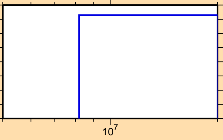
\sigma vs. E for ^{197}\text{Au}(n,t)
