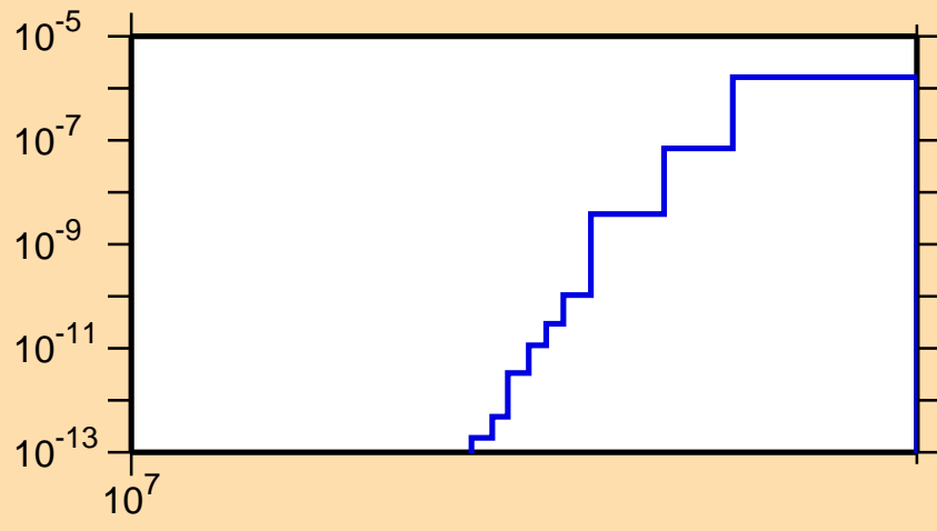
\sigma vs. E for ^{198}\text{Au}(n,nd)
