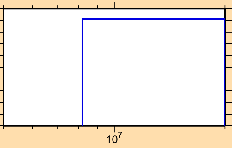
\sigma vs. E for ^{198}\text{Au}(n,t)
