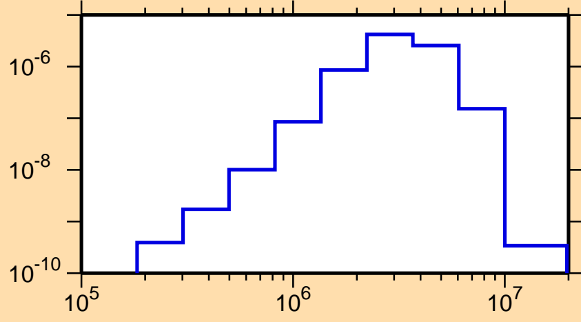
\sigma vs. E for ^{198}\text{Au}(n,n_1)
