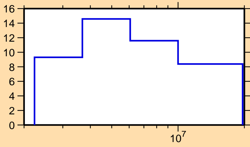
\Delta\sigma/\sigma vs. E for ^{198}\text{Au}(n,el.)
