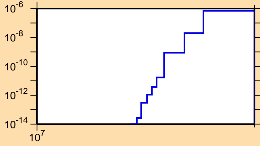
\sigma vs. E for ^{200}\text{Au}(n,nd)
