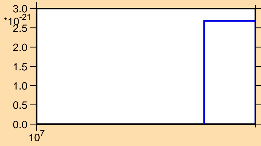
\sigma vs. E for ^{200}\text{Au}(\text{mt } 11)
