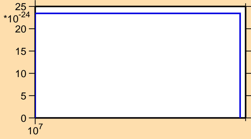
\sigma vs. E for ^{200}\text{Au}(\text{mt } 11)
