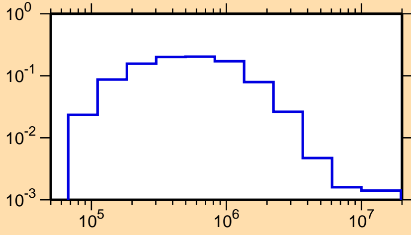
\sigma vs. E for ^{200}\text{Au}(n,n_2)
