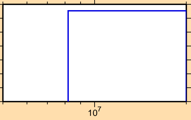
\sigma vs. E for ^{200}\text{Au}(n,nd)
