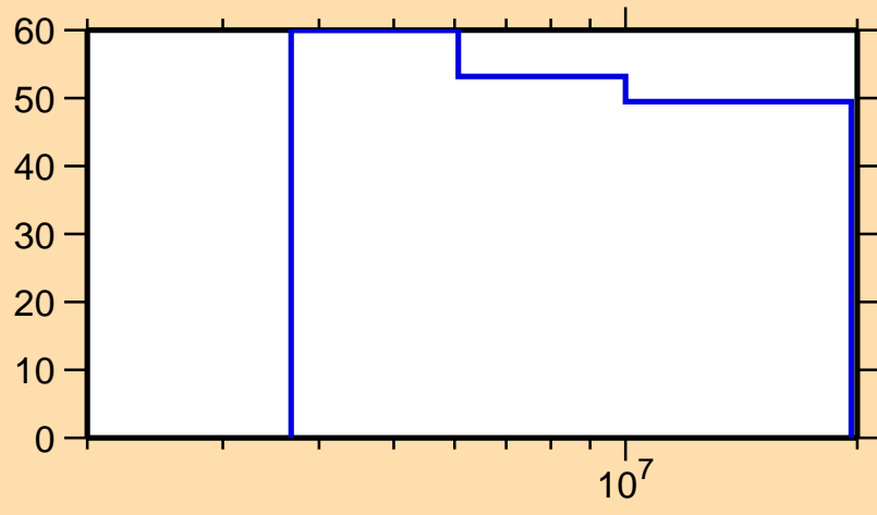
\Delta\sigma/\sigma vs. E for ^{202}\text{Au}(n,p)
