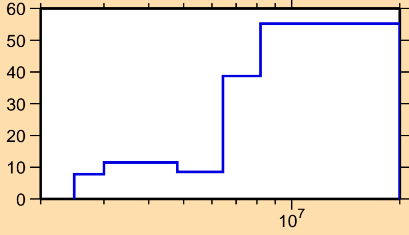
\Delta\sigma/\sigma vs. E for ^{202}\text{Au}(n,n\text{cont.})
