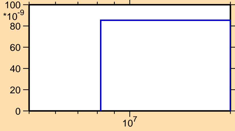
\sigma vs. E for ^{202}\text{Au}(n,n\alpha)
