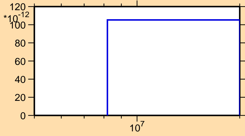
\sigma vs. E for ^{202}\text{Au}(n,2np)
