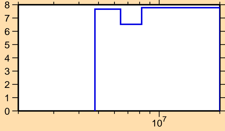
\Delta\sigma/\sigma vs. E for ^{202}\text{Au}(n,\text{nonel.})
