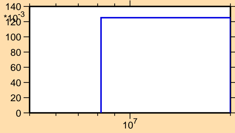
\sigma vs. E for ^{202}\text{Au}(n,3n)
