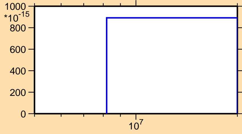
\sigma vs. E for ^{202}\text{Au}(n,2n\alpha)
