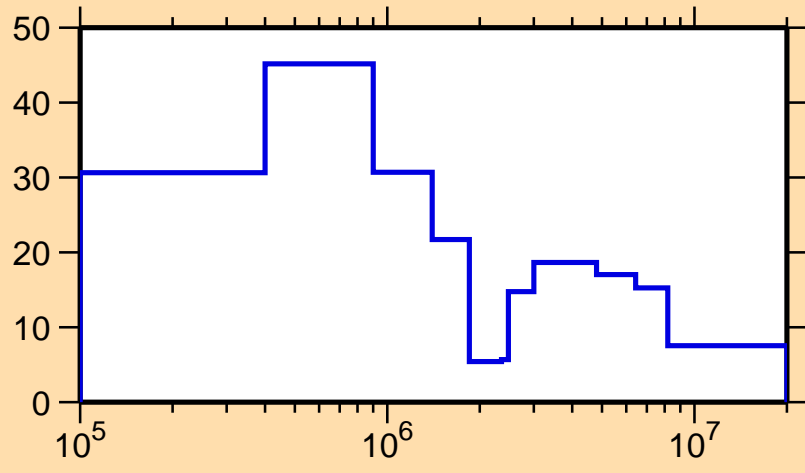
\Delta\sigma/\sigma vs. E for ^{202}\text{Au}(n,\text{tot.})
