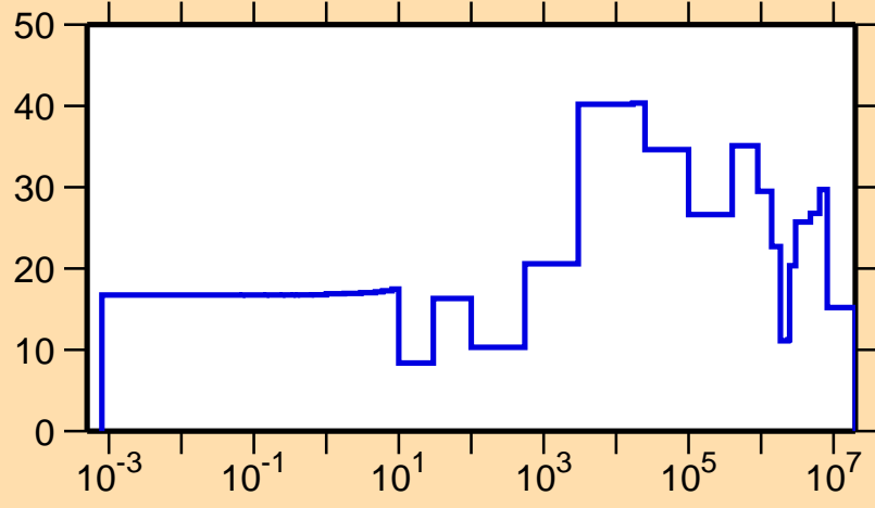
\Delta\sigma/\sigma vs. E for ^{202}\text{Au}(n,\text{el.})
