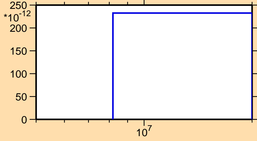
\sigma vs. E for ^{202}\text{Au}(n,nt)
