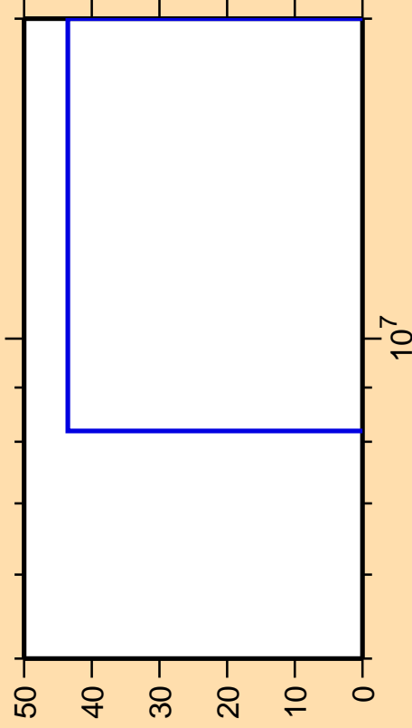
\Delta\sigma/\sigma vs. E for ^{202}\text{Au}(n,3n)
