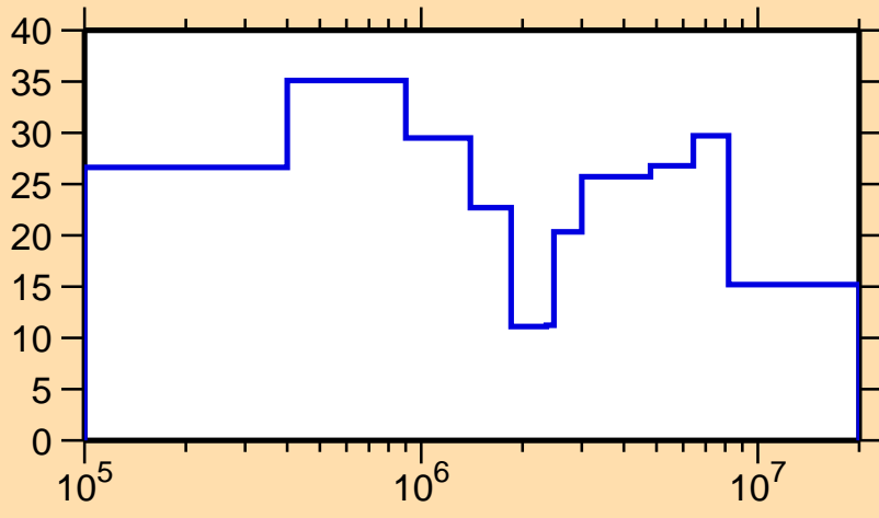
\Delta\sigma/\sigma vs. E for ^{202}\text{Au}(n,\text{el.})
