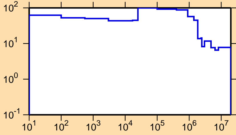
\Delta\sigma/\sigma vs. E for ^{202}\text{Au}(n,\text{nonel.})
