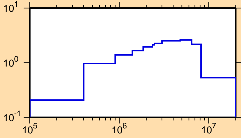
\sigma vs. E for ^{202}\text{Au}(n,n\text{cont.})
