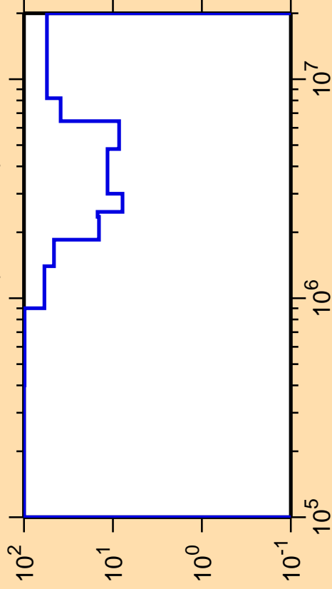
\Delta\sigma/\sigma vs. E for ^{202}\text{Au}(n,n\text{cont.})
