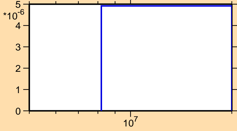
\sigma vs. E for ^{202}\text{Au}(n,t)
