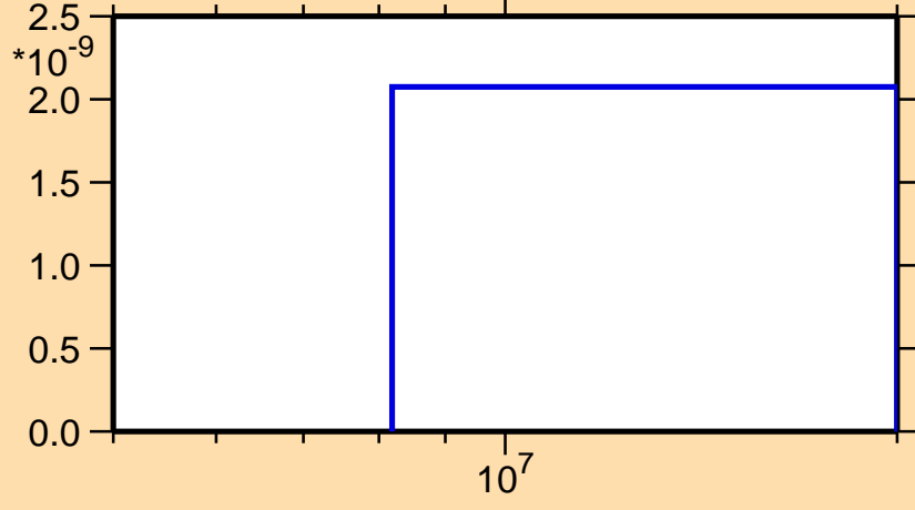
\sigma vs. E for ^{202}\text{Au}(n,nd)
