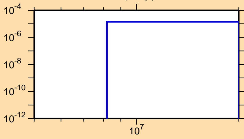
\sigma vs. E for ^{202}\text{Au}(n,np)
