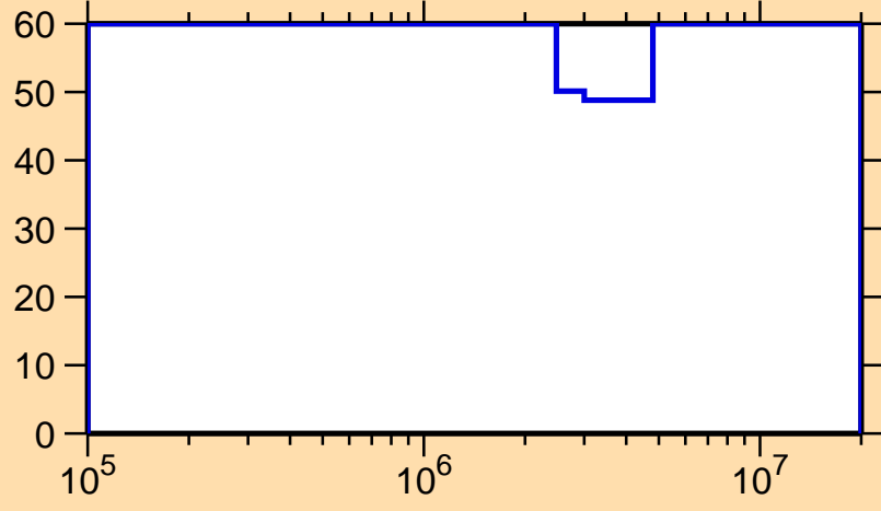
\Delta\sigma/\sigma vs. E for ^{202}\text{Au}(n,n_1)
