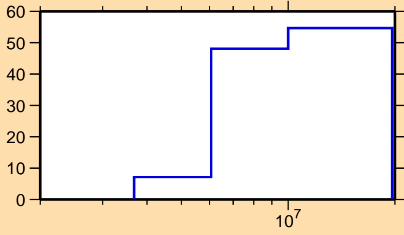
\Delta\sigma/\sigma vs. E for ^{203}\text{Au}(n,p)
