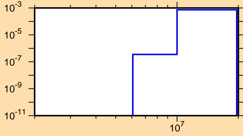
\sigma vs. E for ^{203}\text{Au}(n,p)
