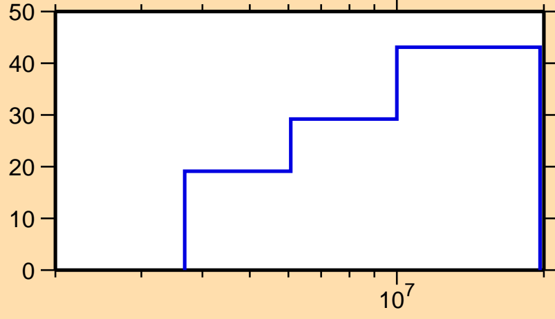
\Delta\sigma/\sigma vs. E for ^{203}\text{Au}(n,n\text{cont.})
