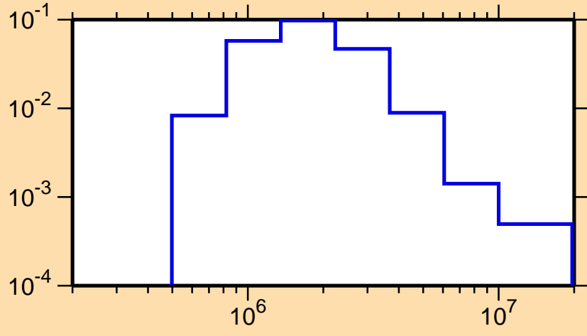
\sigma vs. E for ^{203}\text{Au}(n,n_3)
