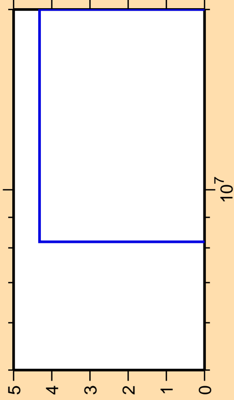
\Delta\sigma/\sigma vs. E for ^{203}\text{Au}(n,2np)
