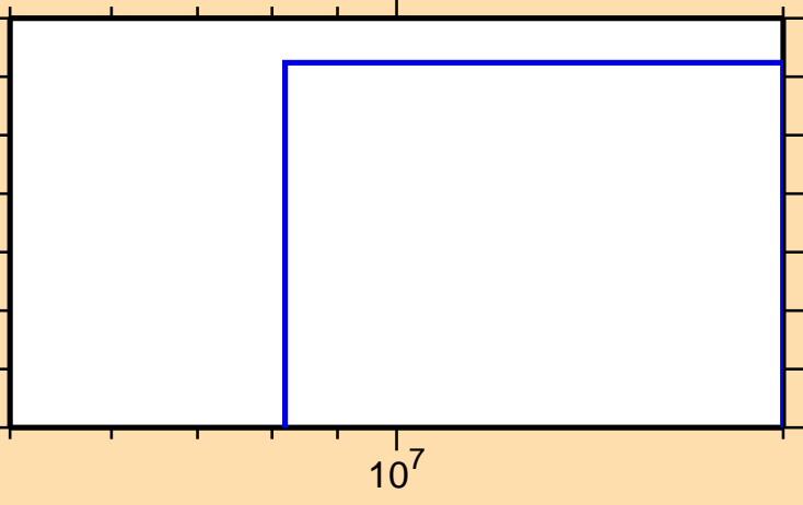
\sigma vs. E for ^{203}\text{Au}(n,2n\alpha)
