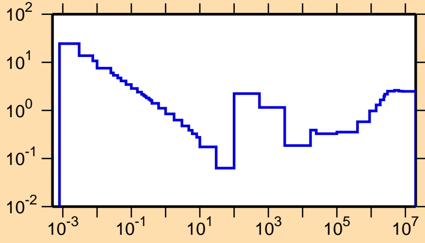
\sigma vs. E for ^{203}\text{Au}(n,\text{nonel.})
