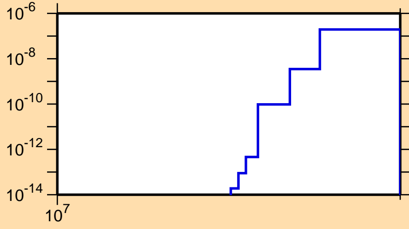
\sigma vs. E for ^{204}\text{Au}(n,nd)
