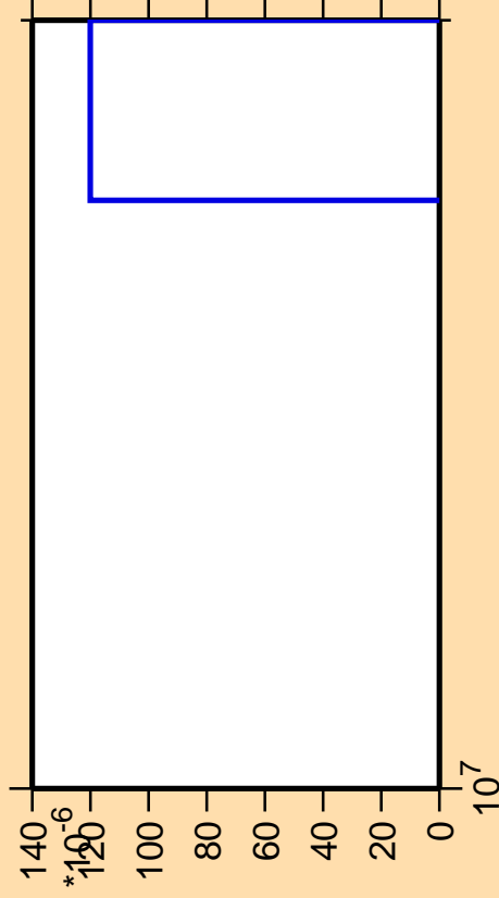
\Delta\sigma/\sigma vs. E for ^{204}\text{Au} (mt 11)
