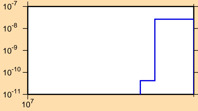
\sigma vs. E for ^{204}\text{Au}(n,nt)
