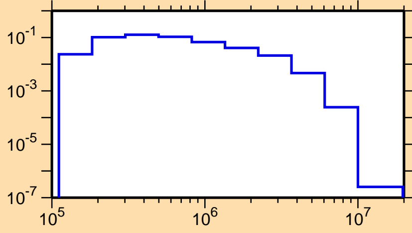
\sigma vs. E for ^{204}\text{Au}(n,n_1)
