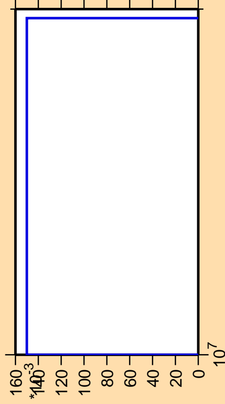
\Delta\sigma/\sigma vs. E for ^{204}\text{Au}(n,2n\alpha)
