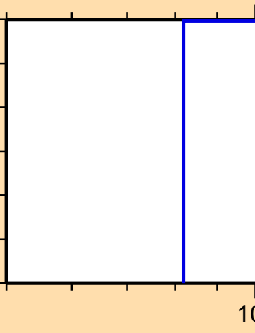
\sigma vs. E for ^{204}\text{Au}(n,np)
