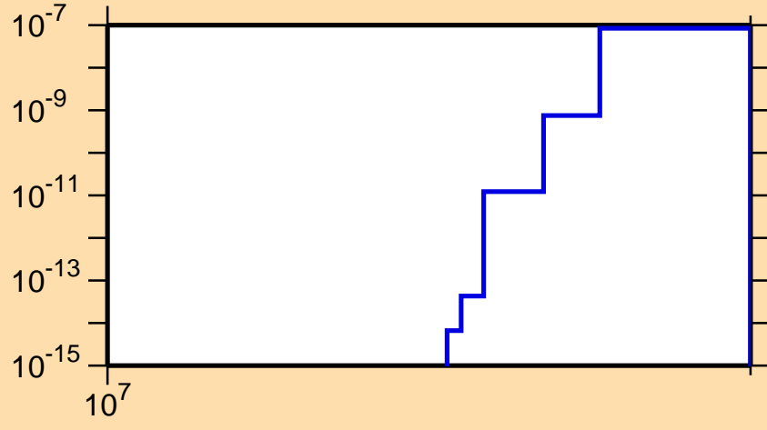
\sigma vs. E for ^{205}\text{Au}(n,nt)
