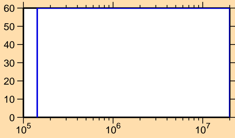
\Delta\sigma/\sigma vs. E for ^{205}\text{Au}(n,n_1)
