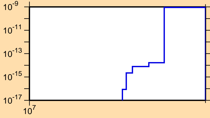
\sigma vs. E for ^{205}\text{Au}(n,2np)
