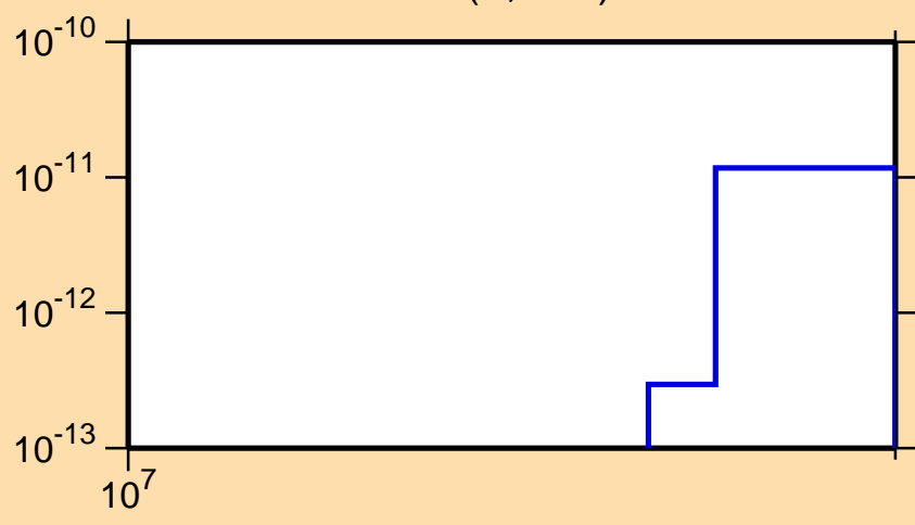
\sigma vs. E for ^{205}\text{Au}(n,2n\alpha)
