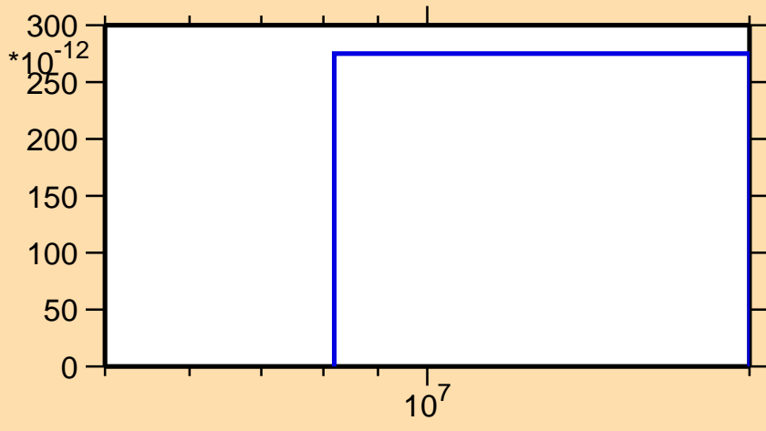
\sigma vs. E for ^{205}\text{Au}(n,\text{nd})
