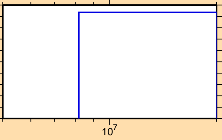
\sigma vs. E for ^{205}\text{Au}(n,d)
