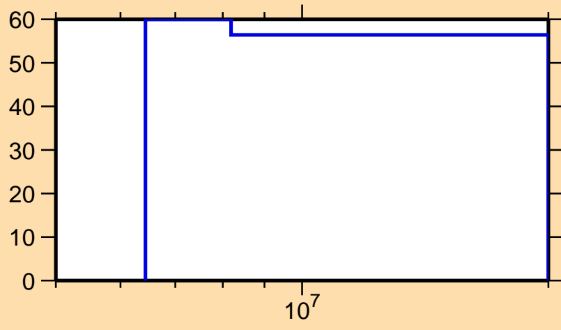
\Delta\sigma/\sigma vs. E for ^{205}\text{Au}(n,n\text{cont.})
