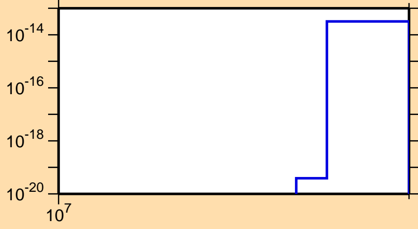
\sigma vs. E for ^{206}\text{Au} (mt 11)
