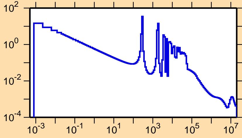
\sigma vs. E for ^{206}\text{Au}(n,\gamma)
