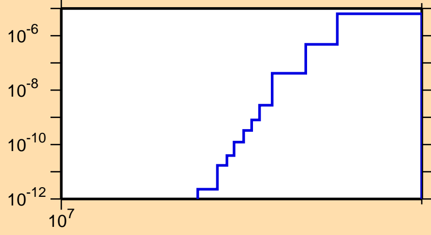
\sigma vs. E for ^{206}\text{Au}(n,\text{nd})
