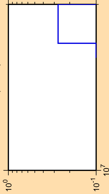
\Delta\sigma/\sigma vs. E for ^{206}\text{Au} (mt 11)
