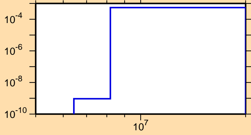
\sigma vs. E for ^{206}\text{Au}(n,p)
