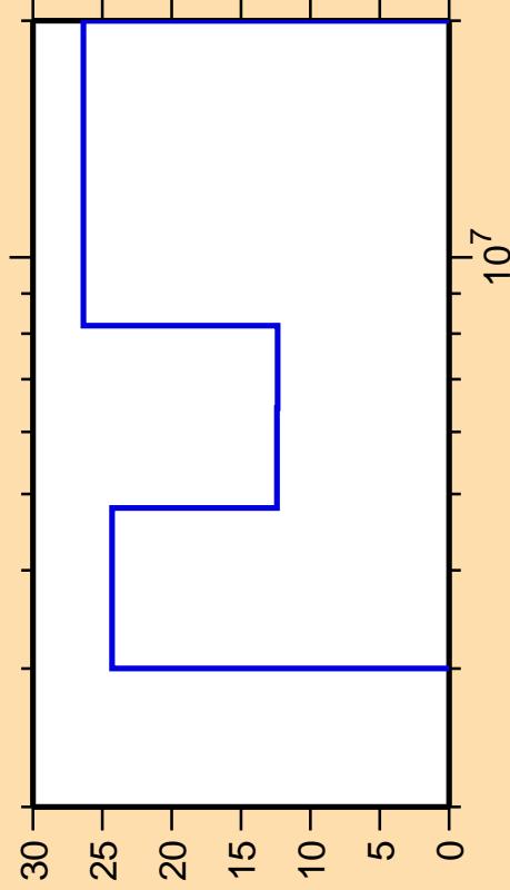
\Delta\sigma/\sigma vs. E for ^{206}\text{Au}(n,2n)
