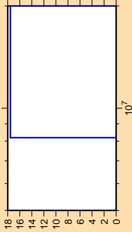
\Delta\sigma/\sigma vs. E for ^{206}\text{Au}(n,3n)
