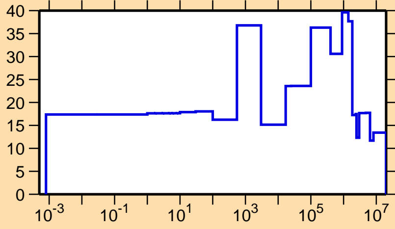
\Delta\sigma/\sigma vs. E for ^{206}\text{Au}(n,\text{el.})
