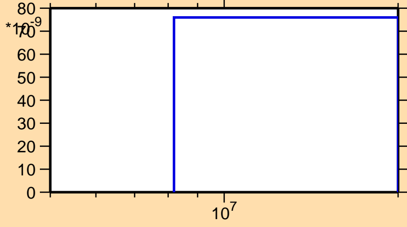
\sigma vs. E for ^{206}\text{Au}(n,nd)
