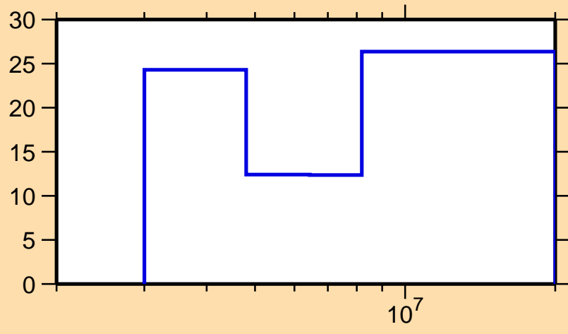
\Delta\sigma/\sigma vs. E for ^{206}\text{Au}(n,2n)
