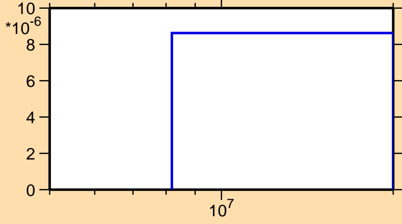
\sigma vs. E for ^{206}\text{Au}(n,np)
