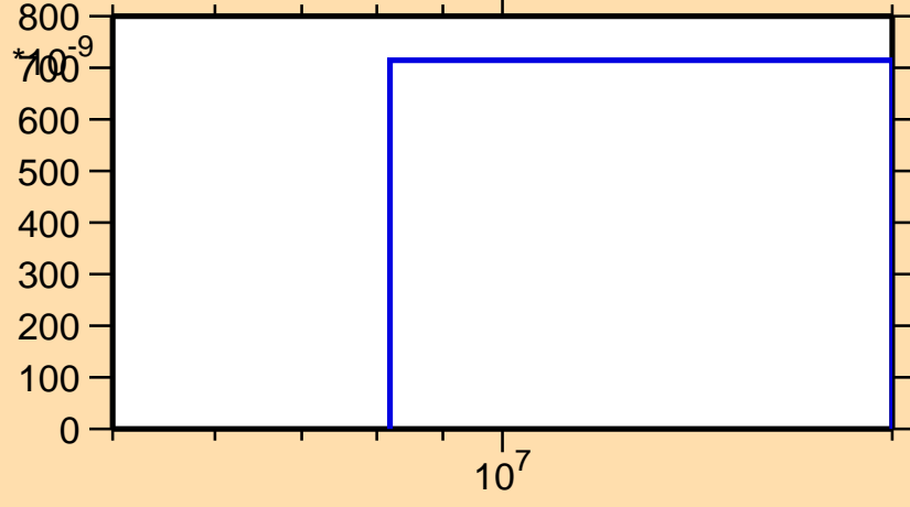
\sigma vs. E for ^{206}\text{Au}(n,n\alpha)
