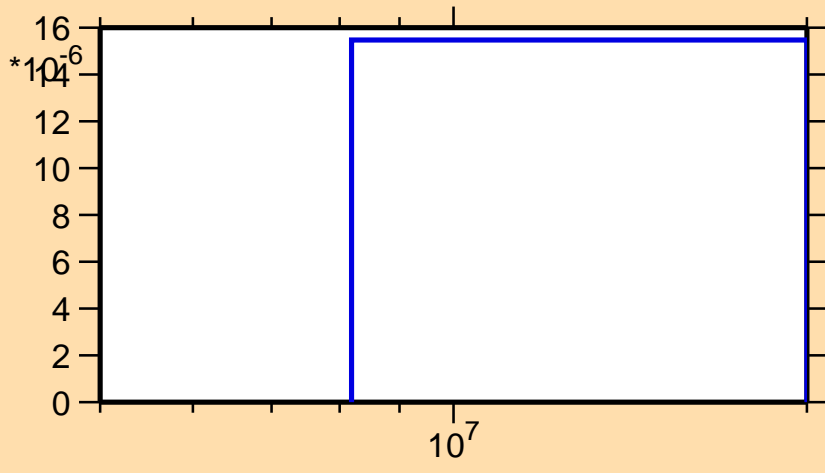
\sigma vs. E for ^{206}\text{Au}(n,d)
