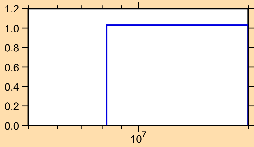
\sigma vs. E for ^{206}\text{Au}(n,3n)
