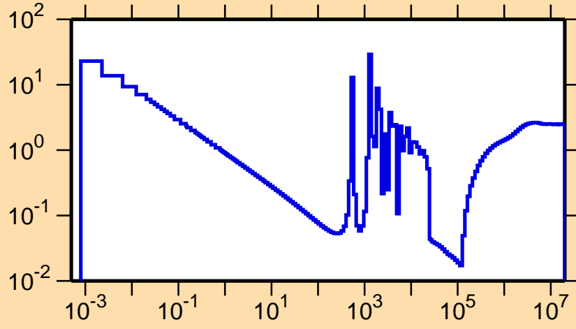
\sigma vs. E for ^{208}\text{Au}(n,\text{nonel.})
