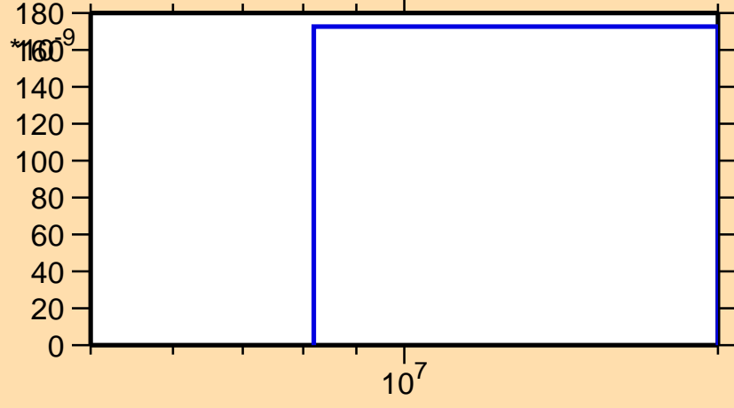
\sigma vs. E for ^{208}\text{Au}(n,nd)
