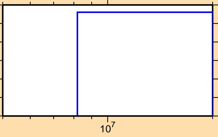
\sigma vs. E for ^{208}\text{Au}(n,2np)
