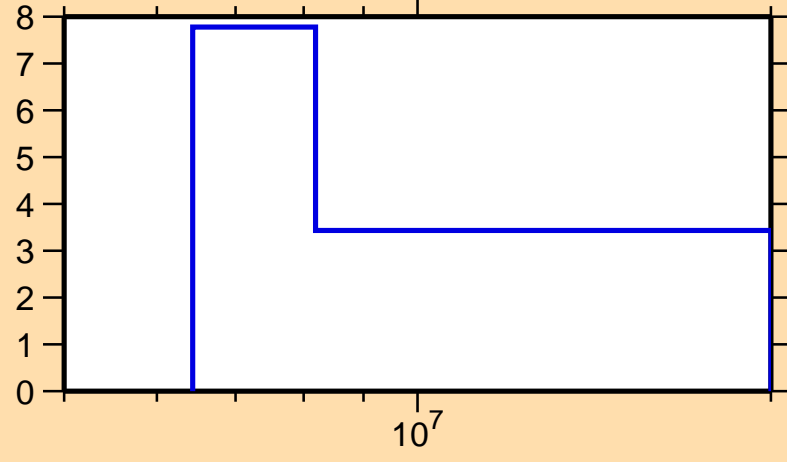
\Delta\sigma/\sigma vs. E for ^{208}\text{Au}(n,\text{tot.})
