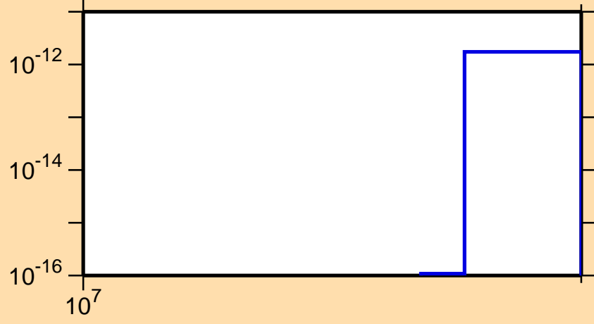
\sigma vs. E for ^{209}\text{Au} (mt 42)
