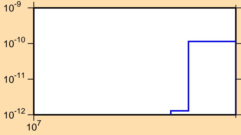
\sigma vs. E for ^{209}\text{Au}(n,3n\alpha)
