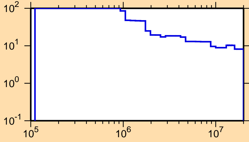
\Delta\sigma/\sigma vs. E for ^{209}\text{Au}(n,\text{nonel.})
