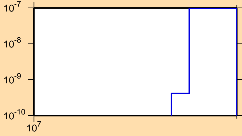
\sigma vs. E for ^{209}\text{Au}(n,2np)
