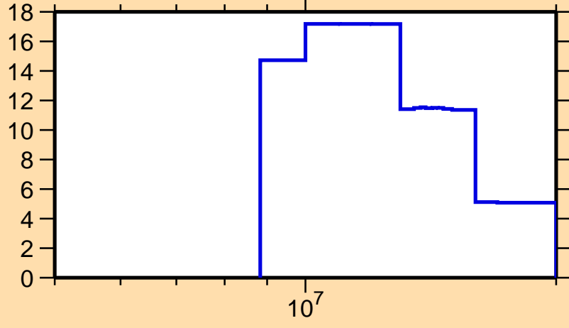
\Delta\sigma/\sigma vs. E for ^{209}\text{Au}(n,el.)
