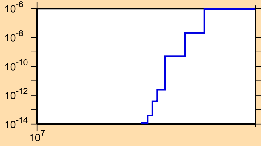
\sigma vs. E for ^{209}\text{Au}(n,\text{nd})
