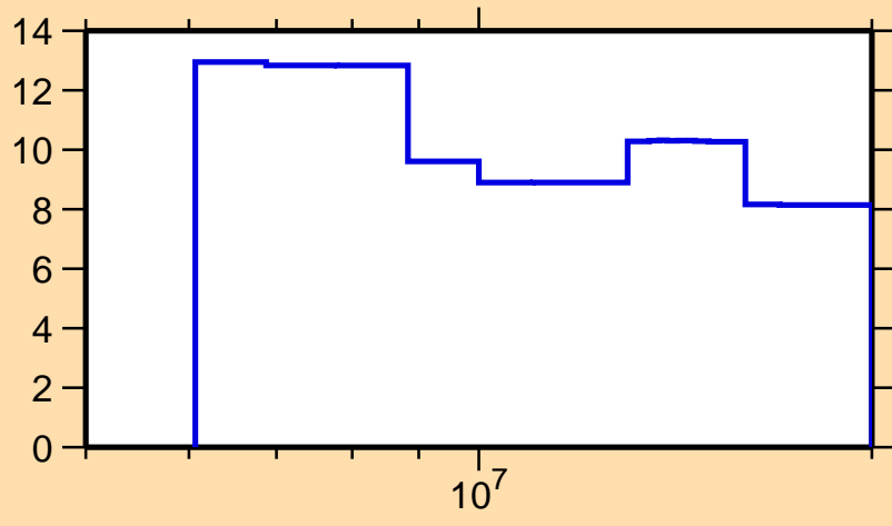
\Delta\sigma/\sigma vs. E for ^{209}\text{Au}(n,\text{nonel.})
