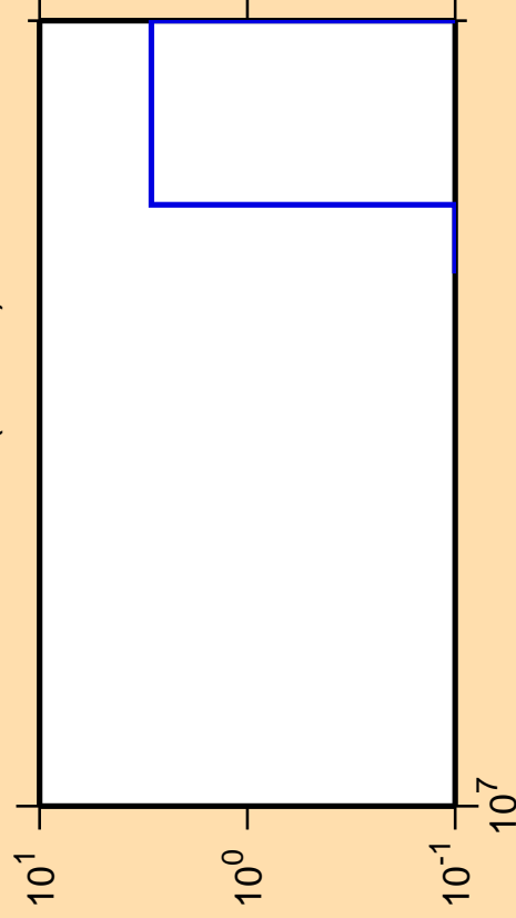
\Delta\sigma/\sigma vs. E for ^{209}\text{Au} (mt 42)
