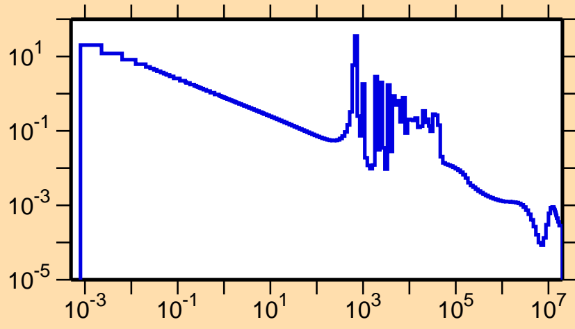
\sigma vs. E for ^{209}\text{Au}(n,\gamma)
