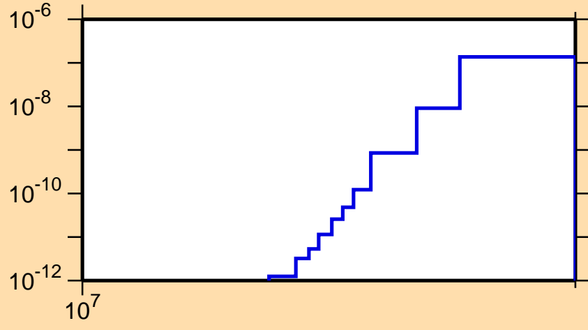
\sigma vs. E for ^{209}\text{Au}(n,2n\alpha)
