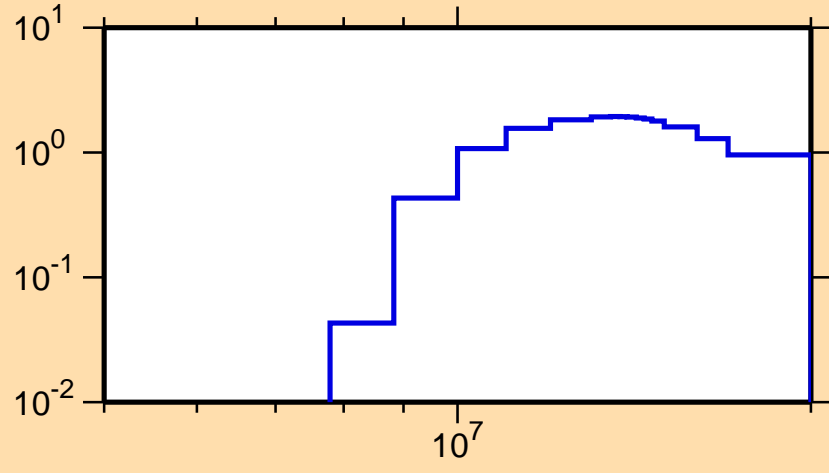
\sigma vs. E for ^{209}\text{Au}(n,3n)
