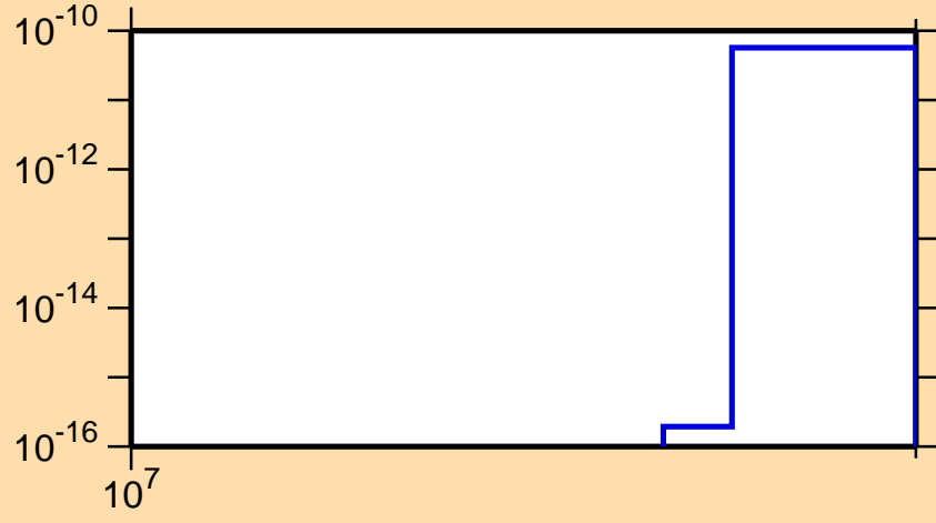
\sigma vs. E for ^{209}\text{Au} (mt 11)
