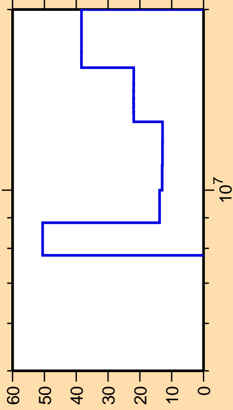
\Delta\sigma/\sigma vs. E for ^{209}\text{Au}(n,3n)
