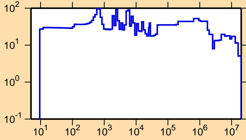
\Delta\sigma/\sigma vs. E for ^{209}\text{Au}(n,\text{el.})
