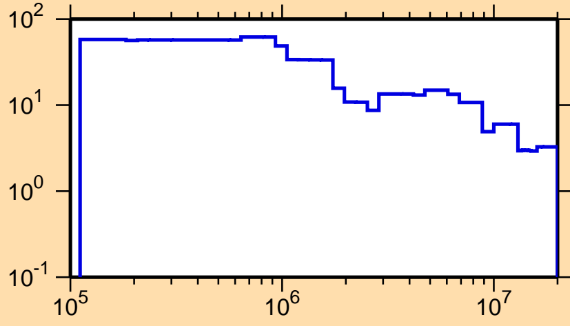
\Delta\sigma/\sigma vs. E for ^{209}\text{Au}(n,\text{tot.})
