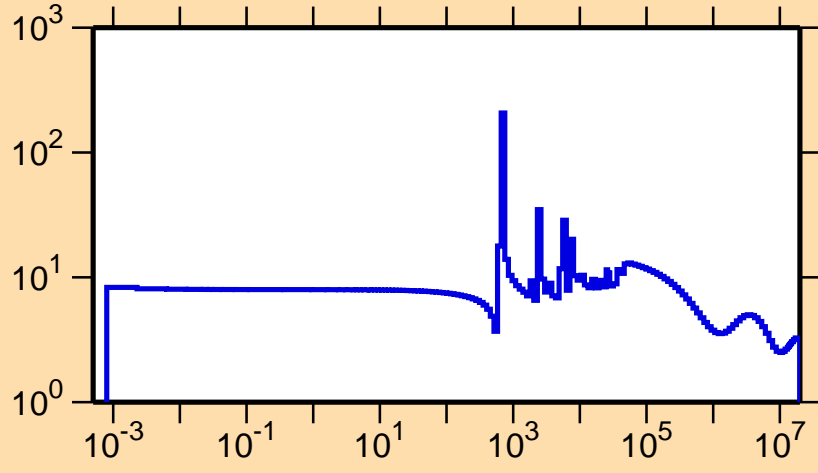
\sigma vs. E for ^{209}\text{Au}(n,\text{el.})
