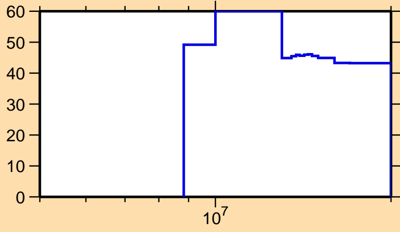
\Delta\sigma/\sigma vs. E for ^{209}\text{Au}(n,2n)
