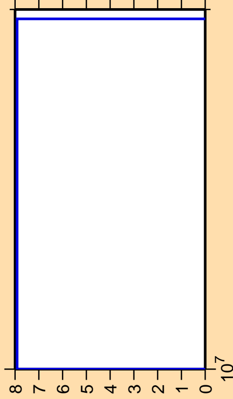
\Delta\sigma/\sigma vs. E for ^{210}\text{Au}(n,3n\alpha)
