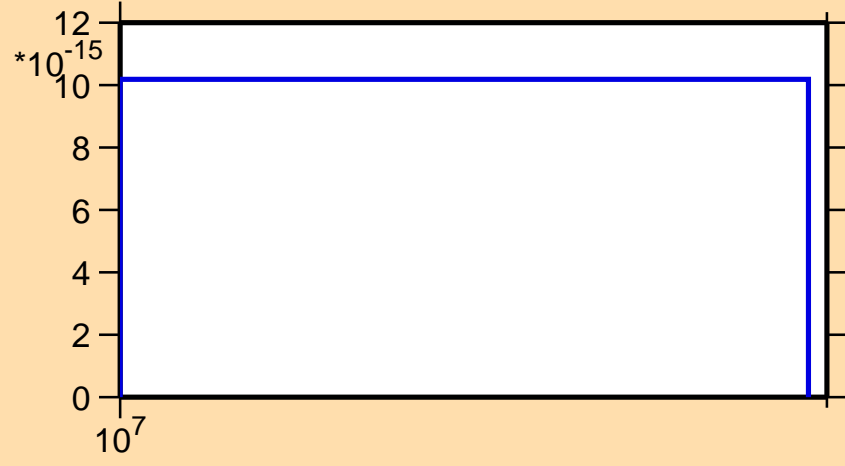
\sigma vs. E for ^{210}\text{Au} (mt 42)
