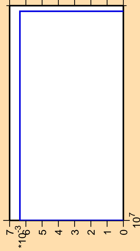
\Delta\sigma/\sigma vs. E for ^{210}\text{Au} (mt 42)
