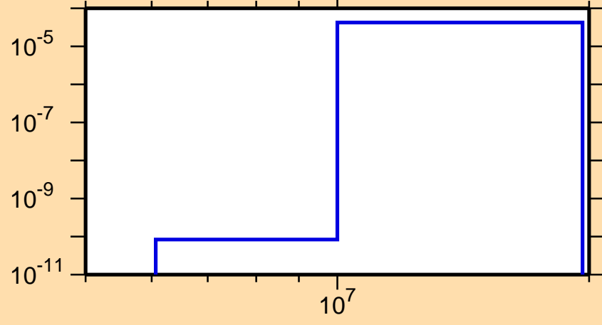
\sigma vs. E for ^{210}\text{Au}(n,t)
