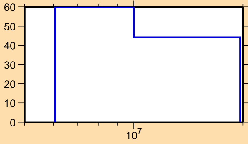
\Delta\sigma/\sigma vs. E for ^{210}\text{Au}(n,n\text{cont.})
