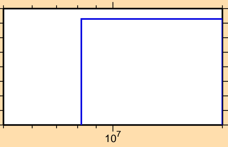
\sigma vs. E for ^{210}\text{Au}(n,d)
