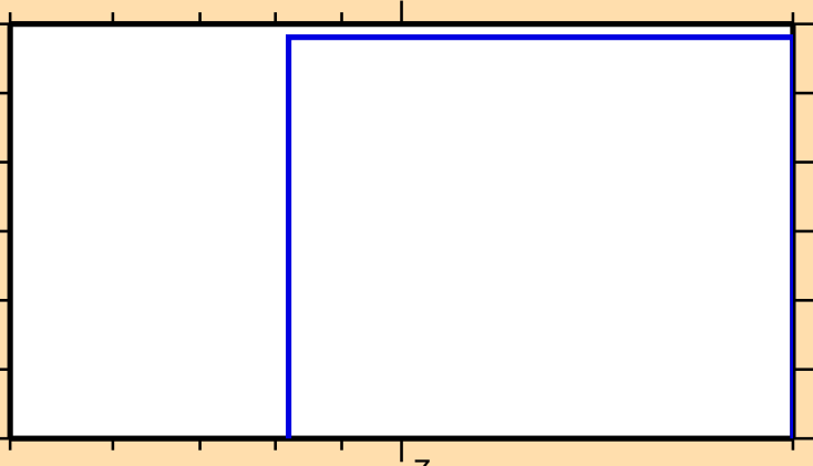
\sigma vs. E for ^{210}\text{Au}(n,2n\alpha)
