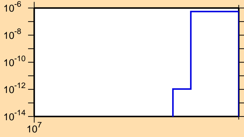
\sigma vs. E for ^{116}\text{Ba}(n,2np)
