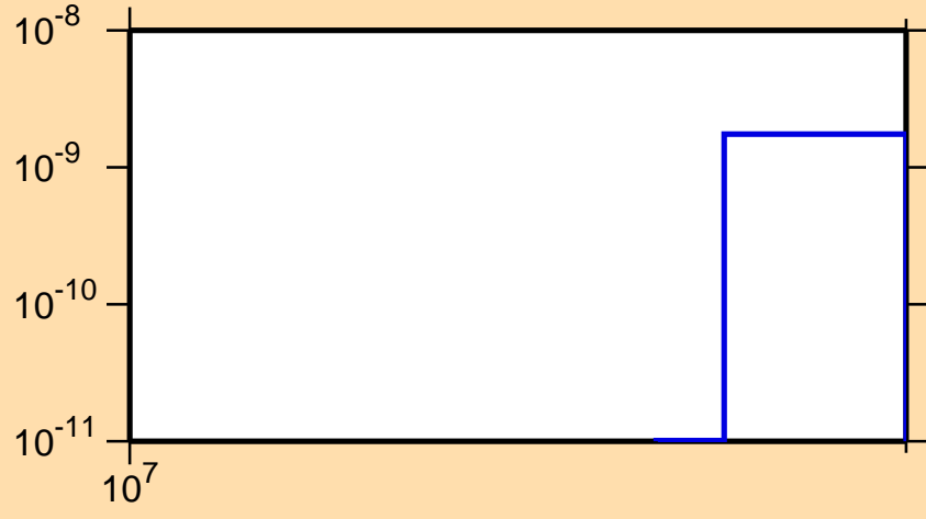
\sigma vs. E for ^{116}\text{Ba}(n,\text{nd})
