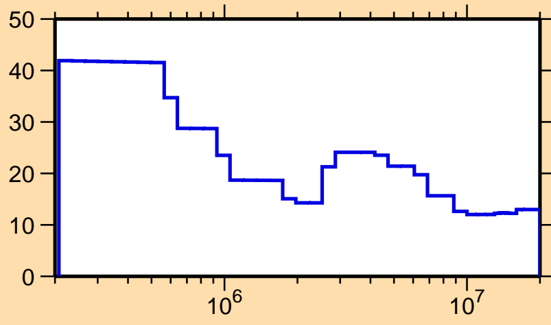
\Delta\sigma/\sigma vs. E for ^{116}\text{Ba}(n,\text{nonel.})
