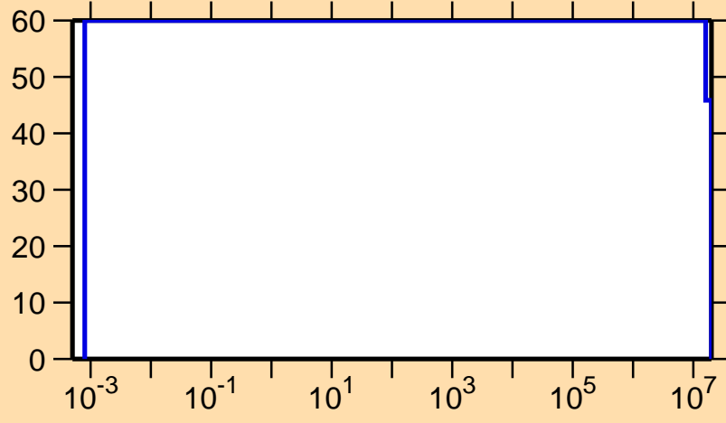
\Delta\sigma/\sigma vs. E for ^{116}\text{Ba}(n,\gamma)
