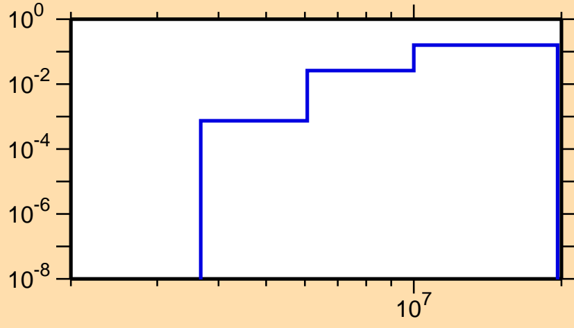
\sigma vs. E for ^{116}\text{Ba}(n,np)
