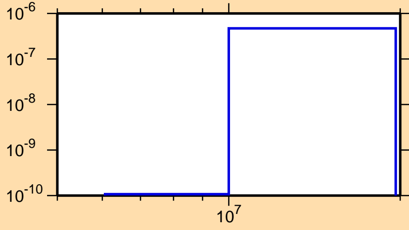
\sigma vs. E for ^{116}\text{Ba}(\text{mt117})
