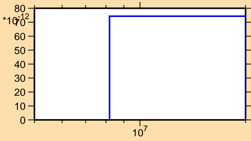
\sigma vs. E for ^{116}\text{Ba}(\text{mt } 34)
