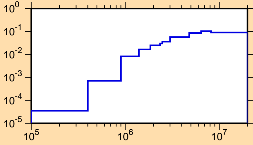
\sigma vs. E for ^{116}\text{Ba}(n,n\text{cont.})
