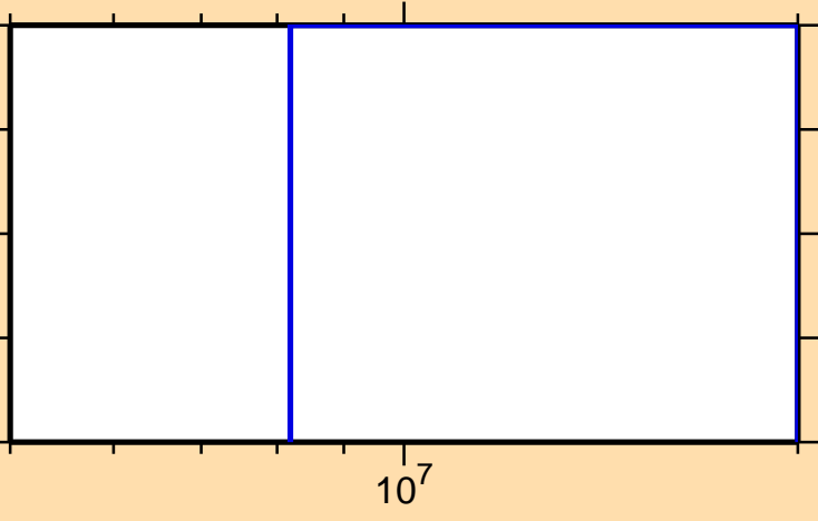
\sigma vs. E for ^{116}\text{Ba}(n,t)
