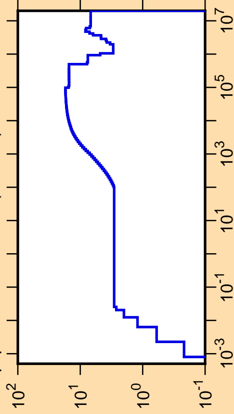
\Delta\mu/\mu vs. E for ^{117}\text{Ba}(\text{mt251})
