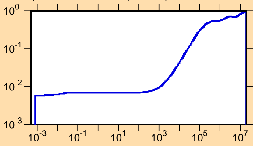
\mu vs. E for ^{117}\text{Ba}(\text{mt251})
