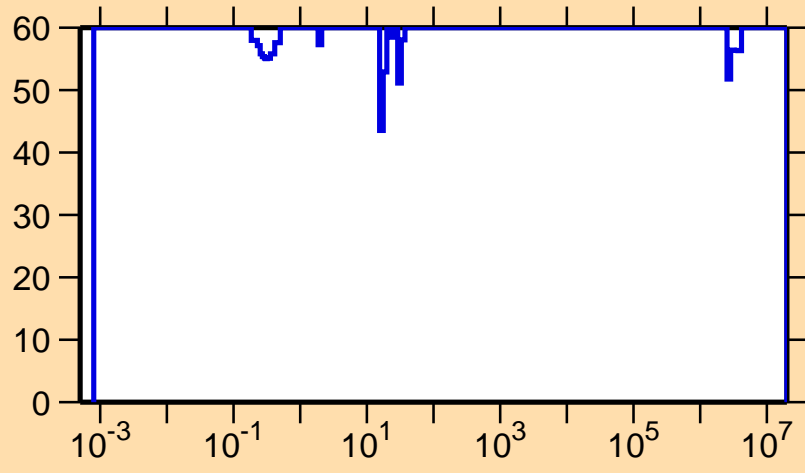
\Delta\sigma/\sigma vs. E for ^{117}\text{Ba}(n,\gamma)
