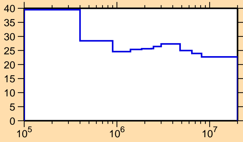
\Delta\sigma/\sigma vs. E for ^{117}\text{Ba}(n,n_1)
