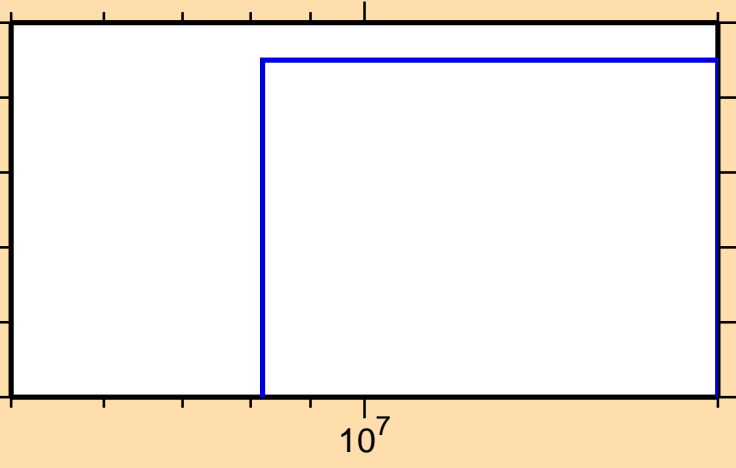
\sigma vs. E for ^{117}\text{Ba}(n,\text{nd})
