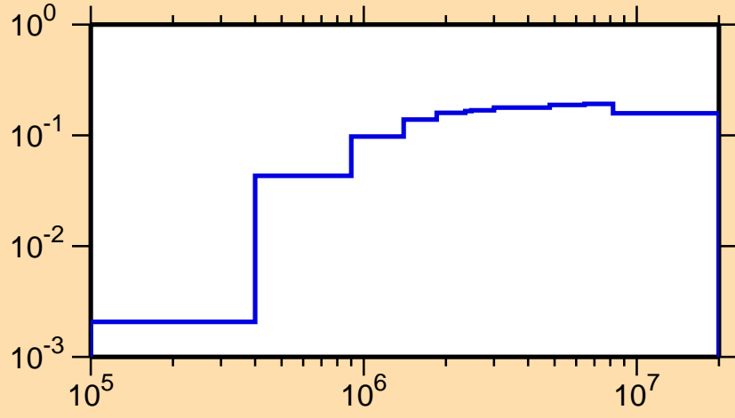
\sigma vs. E for ^{117}\text{Ba}(n,\text{inel.})
