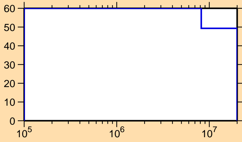
\Delta\sigma/\sigma vs. E for ^{117}\text{Ba}(n,n\text{cont.})
