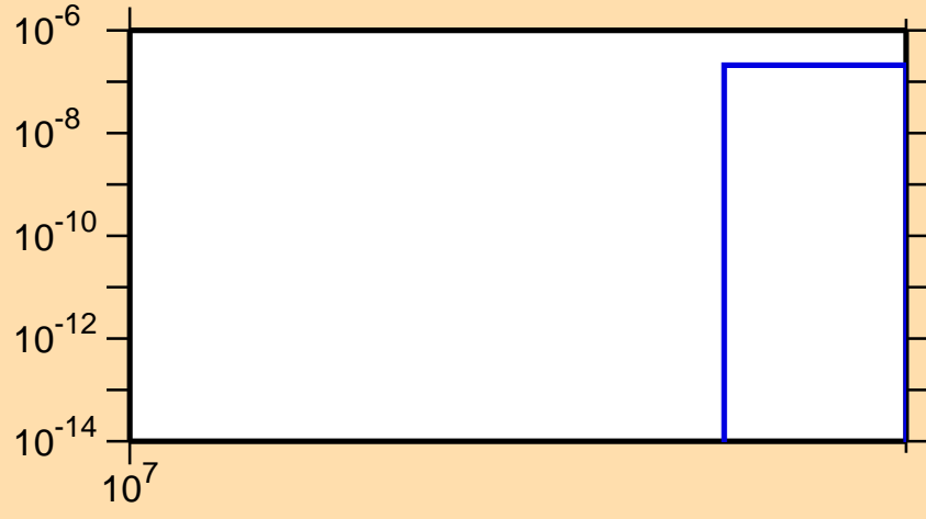
\sigma vs. E for ^{118}\text{Ba}(n,2np)
