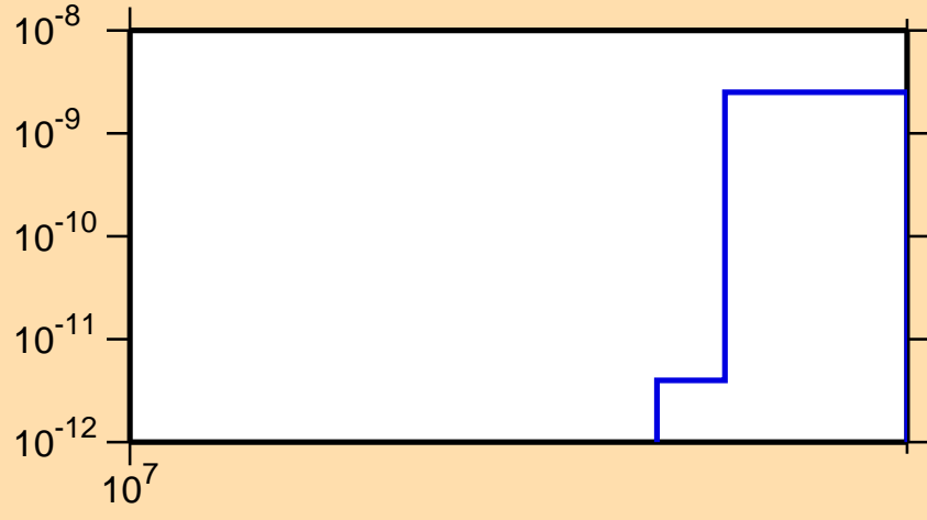
\sigma vs. E for ^{118}\text{Ba}(n,\text{nd})
