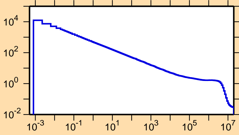
\sigma vs. E for ^{118}\text{Ba}(n,p)
