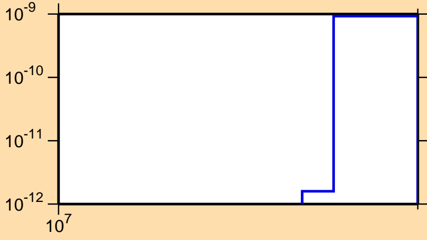
\sigma vs. E for ^{118}\text{Ba}(n,2n\alpha)
