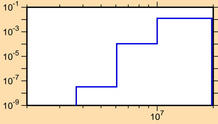
\sigma vs. E for ^{118}\text{Ba}(n,d)
