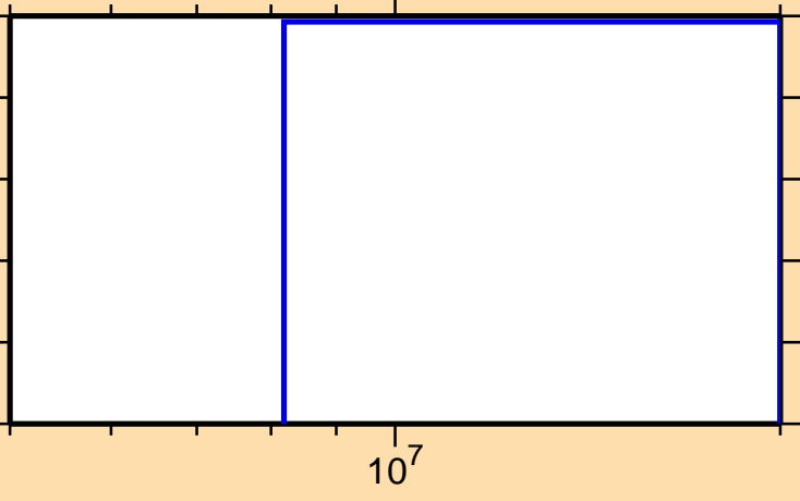
\sigma vs. E for ^{118}\text{Ba}(\text{mt } 45)
