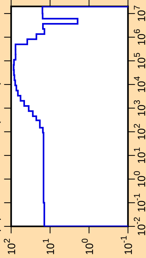
\Delta\mu/\mu vs. E for ^{119}\text{Ba}(\text{mt251})
