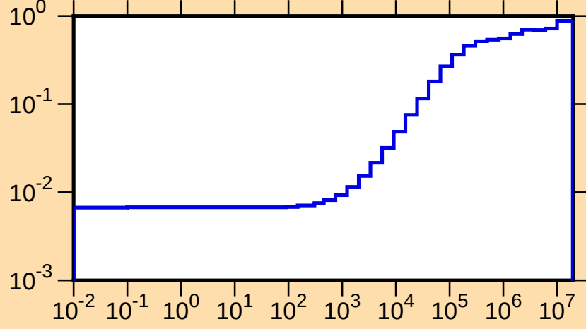
\mu vs. E for ^{119}\text{Ba}(\text{mt251})
