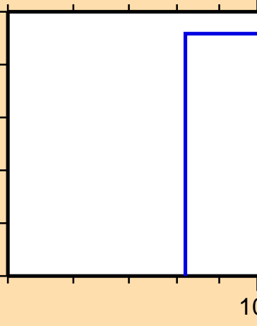
\sigma vs. E for ^{120}\text{Ba}(n,2n)
