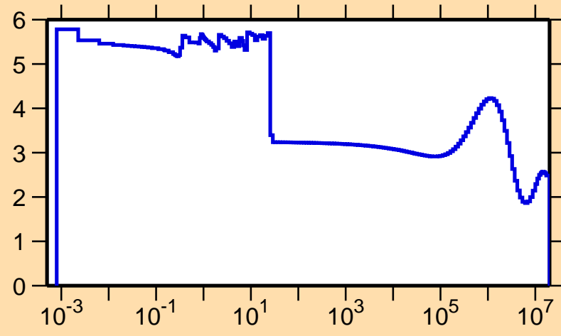
\sigma vs. E for ^{121}\text{Ba}(n,\text{el.})
