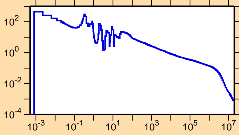
\sigma vs. E for ^{121}\text{Ba}(n,\gamma)
