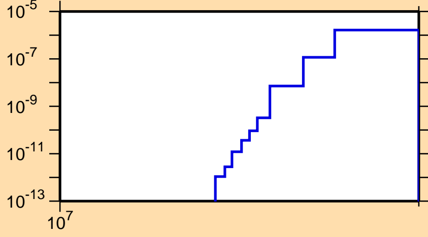
\sigma vs. E for ^{121}\text{Ba}(n,2n\alpha)
