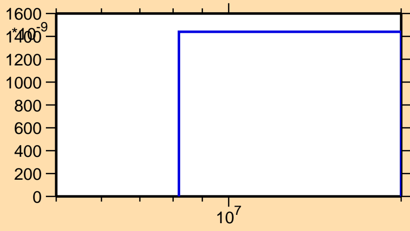
\sigma vs. E for ^{121}\text{Ba}(n,\text{pt})
