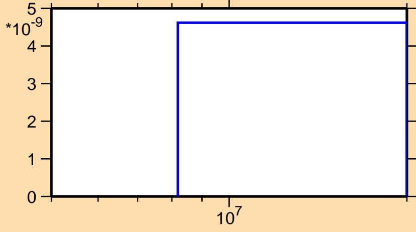
\sigma vs. E for ^{121}\text{Ba}(\text{mt117})
