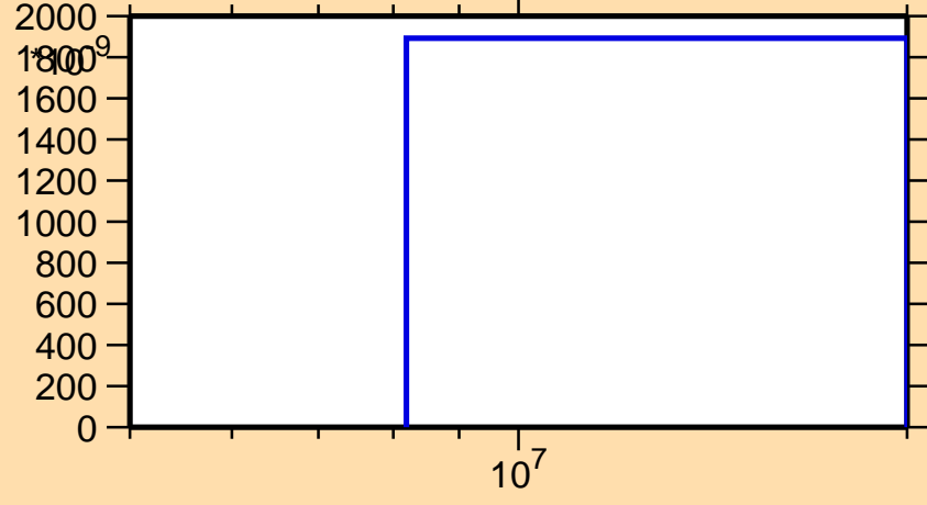
\sigma vs. E for ^{121}\text{Ba}(n,2np)
