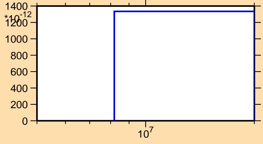
\sigma vs. E for ^{121}\text{Ba} (mt 34)
