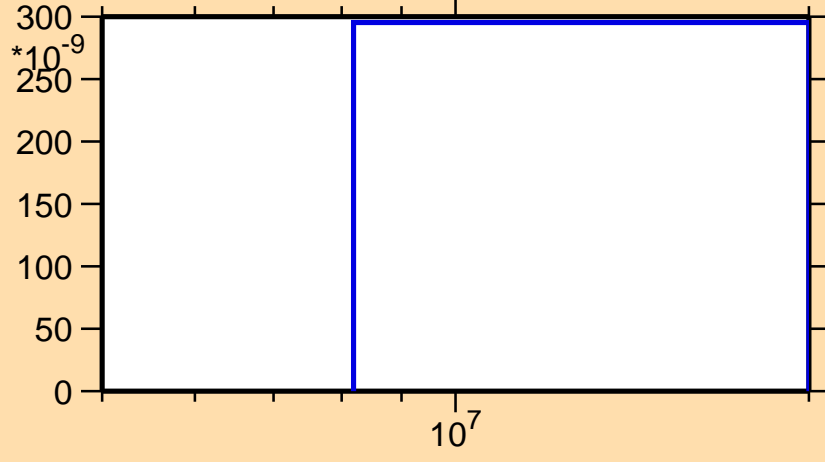
\sigma vs. E for ^{121}\text{Ba} (mt 45)
