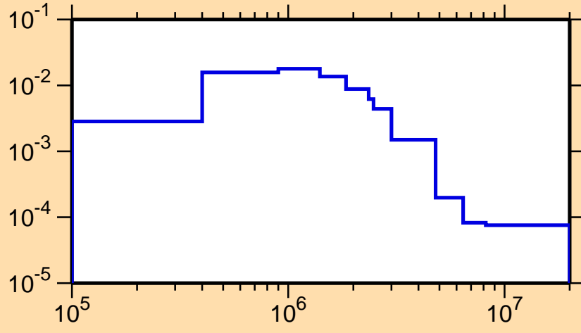
\sigma vs. E for ^{121}\text{Ba}(n,n_4)
