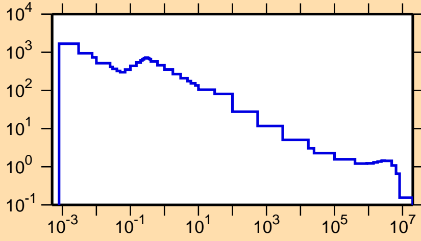
\sigma vs. E for ^{121}\text{Ba}(n,p)
