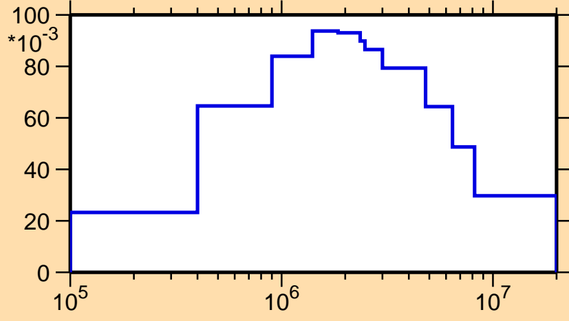
\sigma vs. E for ^{121}\text{Ba}(n,n_2)
