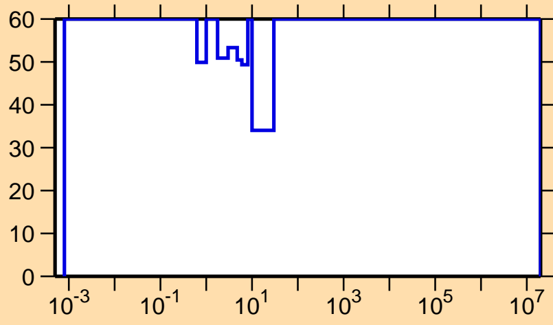
\Delta\sigma/\sigma vs. E for ^{121}\text{Ba}(n,\gamma)
