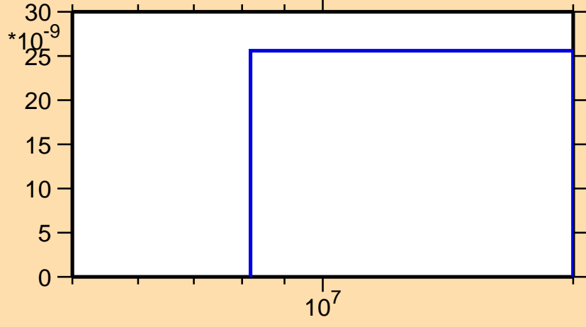
\sigma vs. E for ^{121}\text{Ba}(n,\text{nd})
