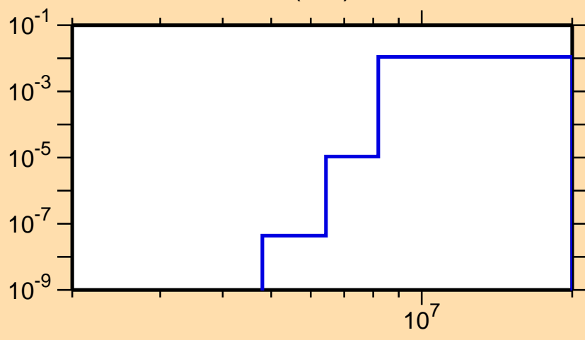
\sigma vs. E for ^{121}\text{Ba}(n,d)
