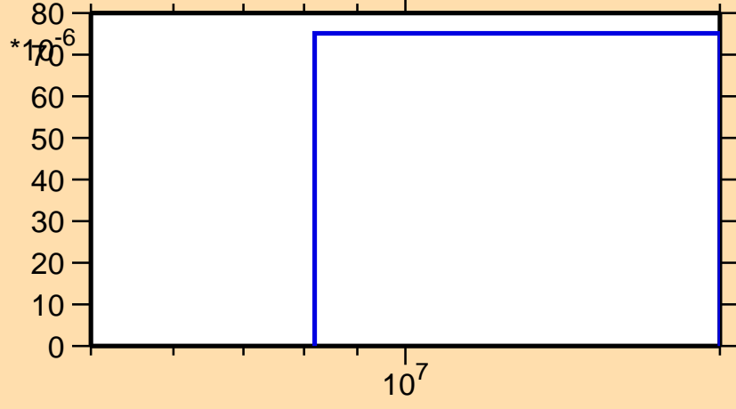
\sigma vs. E for ^{121}\text{Ba}(n,\text{pd})
