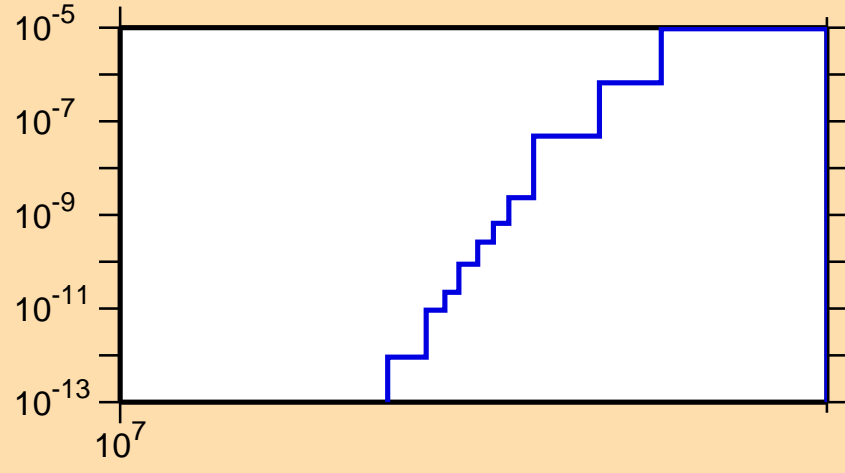
\sigma vs. E for ^{123}\text{Ba}(n,\text{pt})
