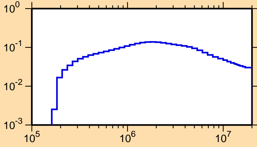
\sigma vs. E for ^{123}\text{Ba}(n,n_4)
