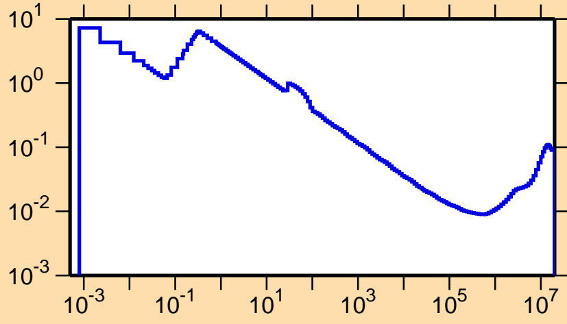
\sigma vs. E for ^{123}\text{Ba}(n,\alpha)
